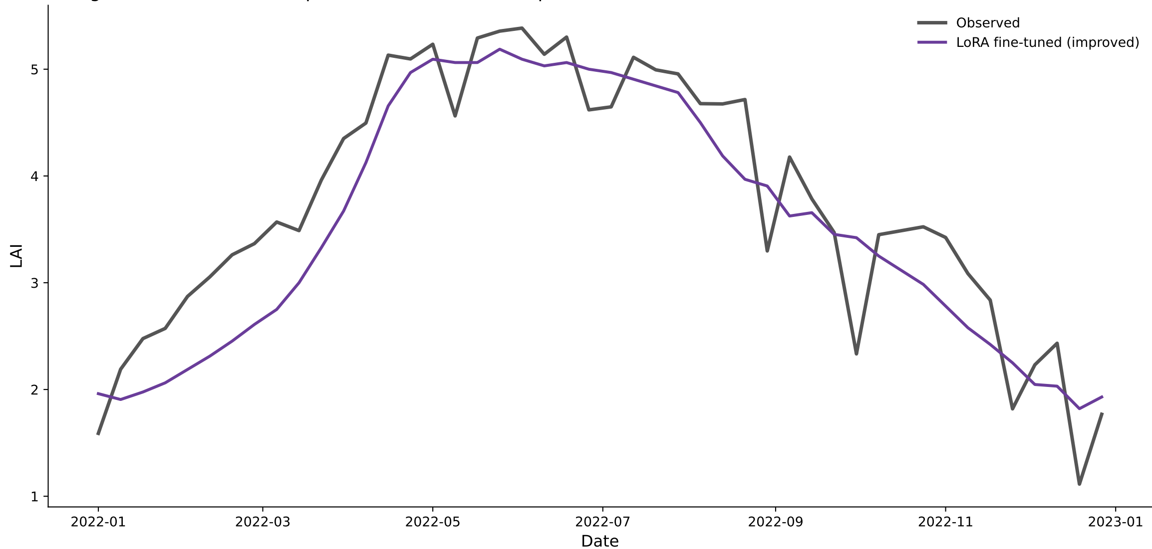
evergreen — Chronos-2 (improved LoRA fine-tuned) predicted vs. observed LAI, 2022
