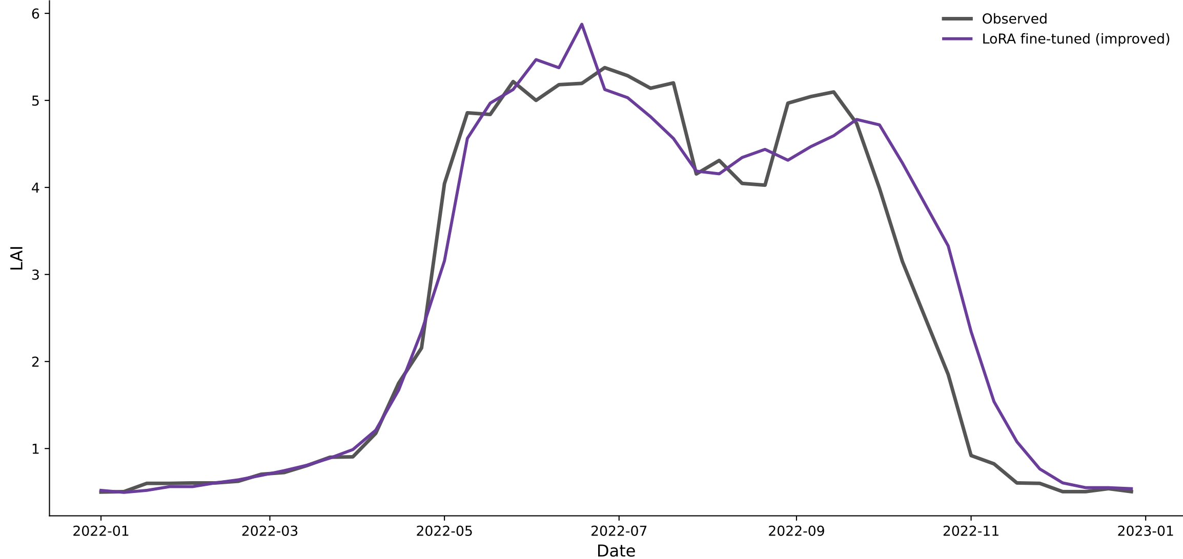
high_amplitude_deciduous — Chronos-2 (improved LoRA fine-tuned) predicted vs. observed LAI, 2022
