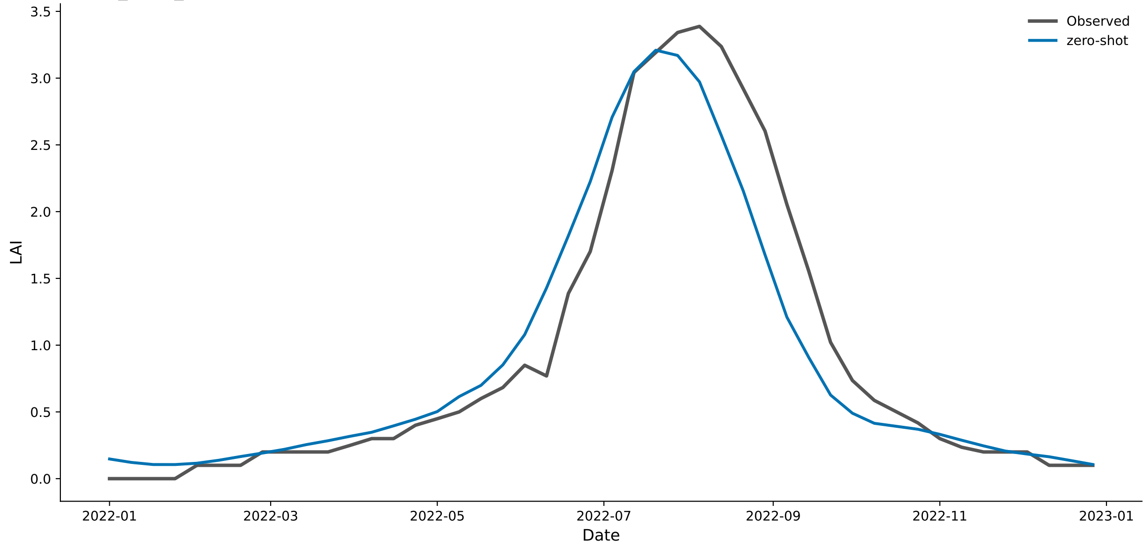
px018_trees_nd — Chronos-2 (zero-shot) predicted vs. observed LAI, 2022
