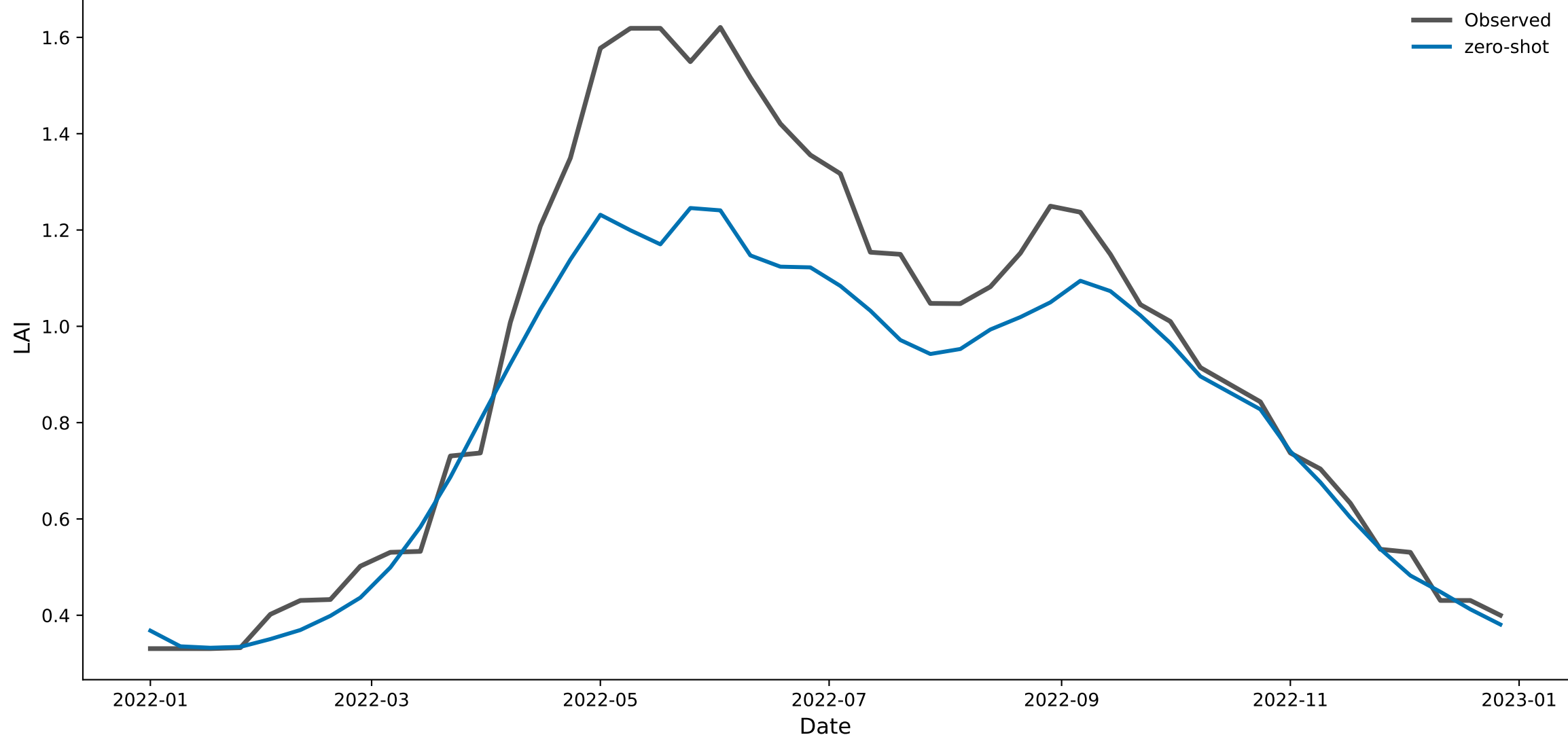
px019_shrubs_bd — Chronos-2 (zero-shot) predicted vs. observed LAI, 2022
