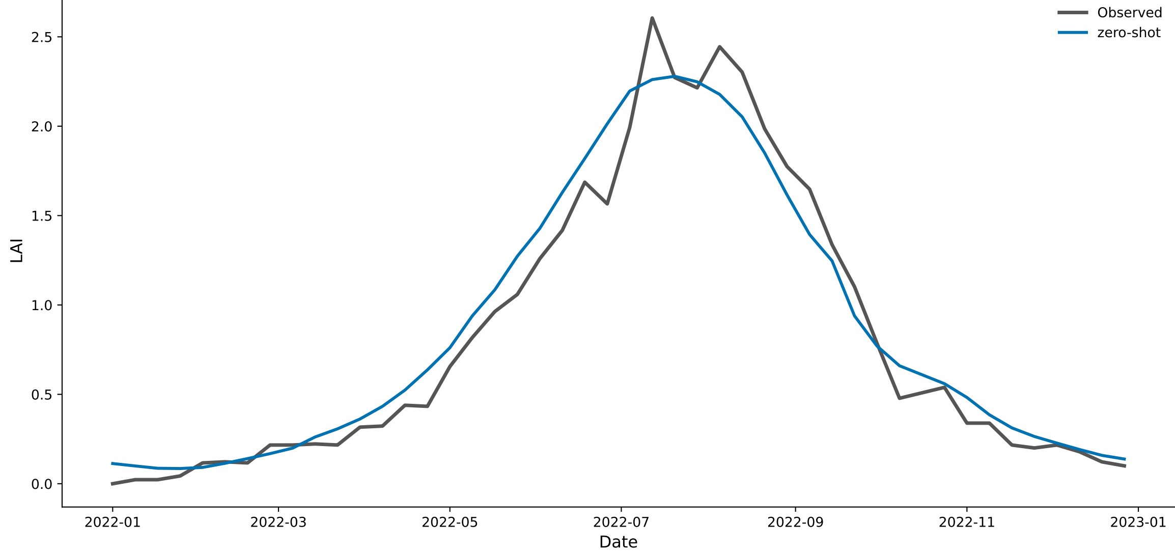
px022_grass_nat — Chronos-2 (zero-shot) predicted vs. observed LAI, 2022
