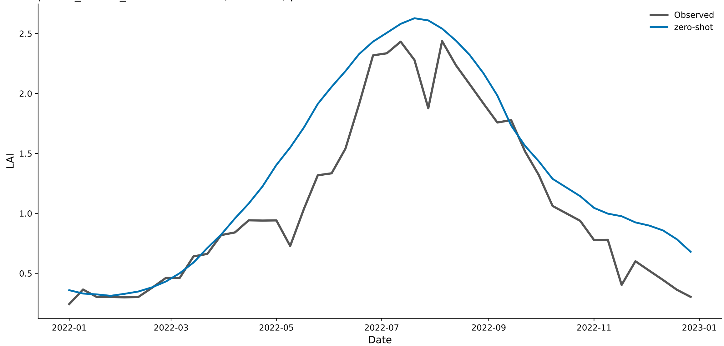
px023_shrubs_ne — Chronos-2 (zero-shot) predicted vs. observed LAI, 2022
