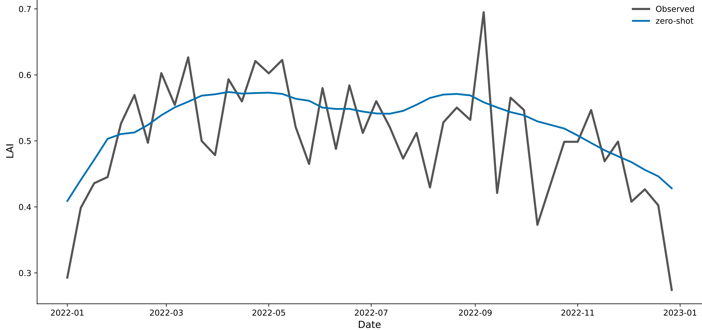
px025_grass_nat — Chronos-2 (zero-shot) predicted vs. observed LAI, 2022
