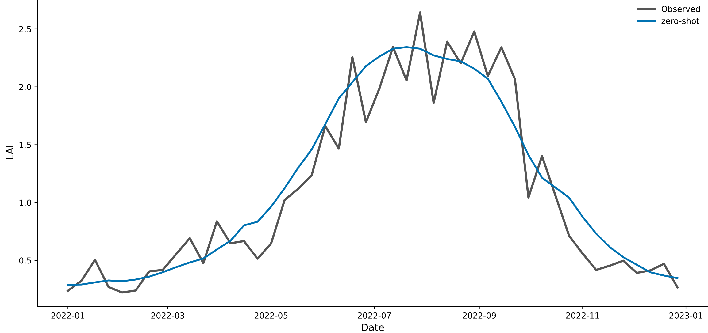
px038_grass_nat — Chronos-2 (zero-shot) predicted vs. observed LAI, 2022
