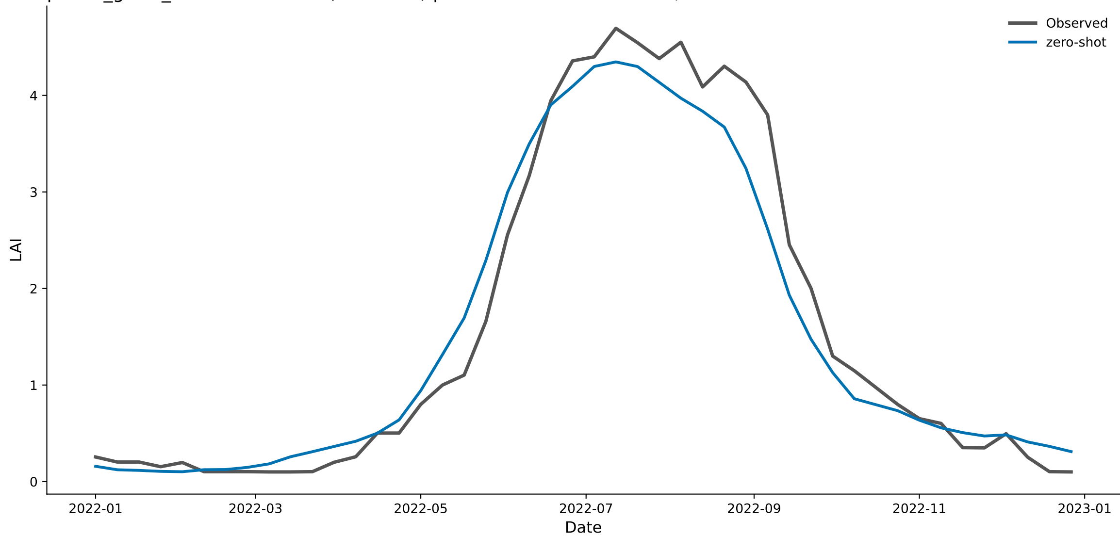
px042_grass_nat — Chronos-2 (zero-shot) predicted vs. observed LAI, 2022
