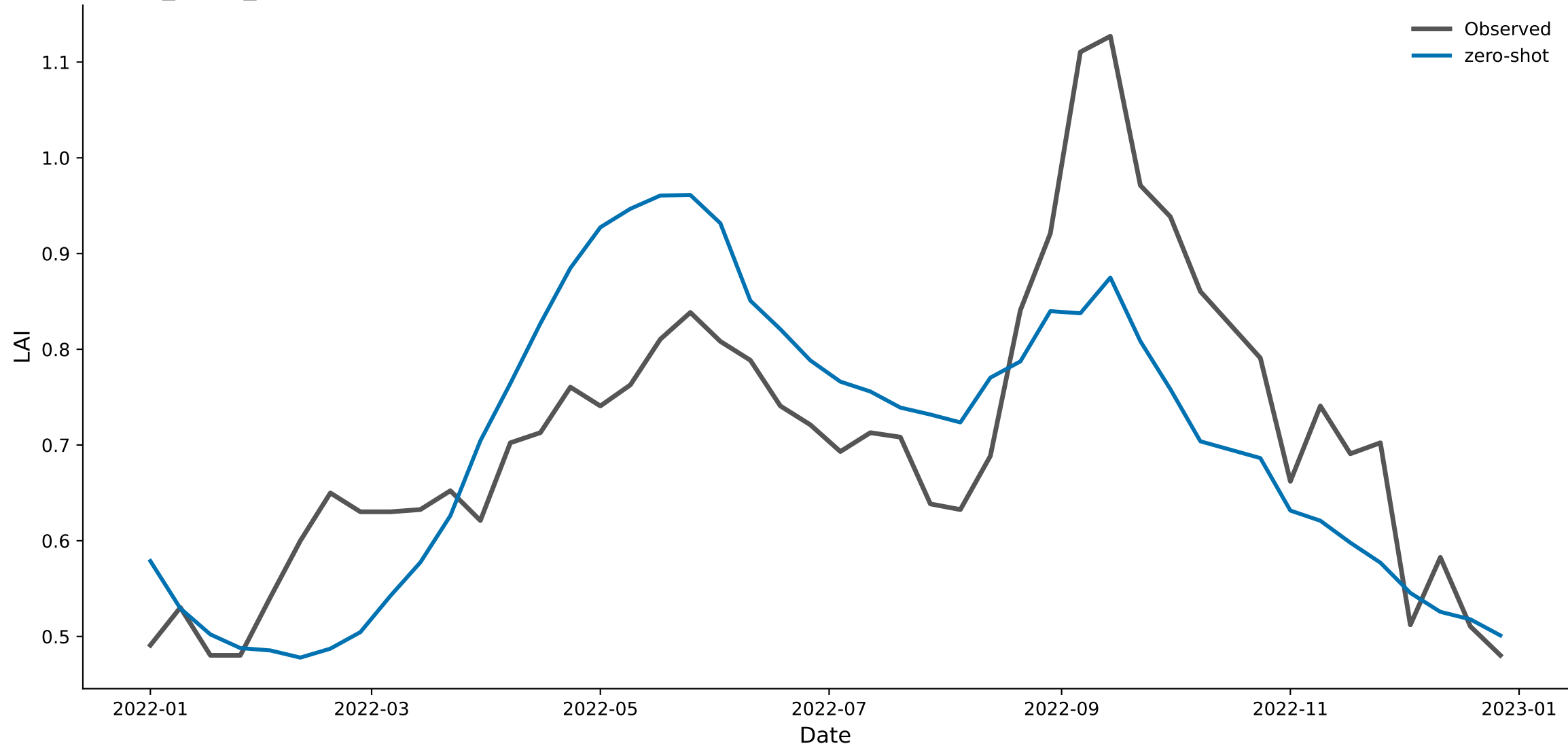
px049_grass_nat — Chronos-2 (zero-shot) predicted vs. observed LAI, 2022
