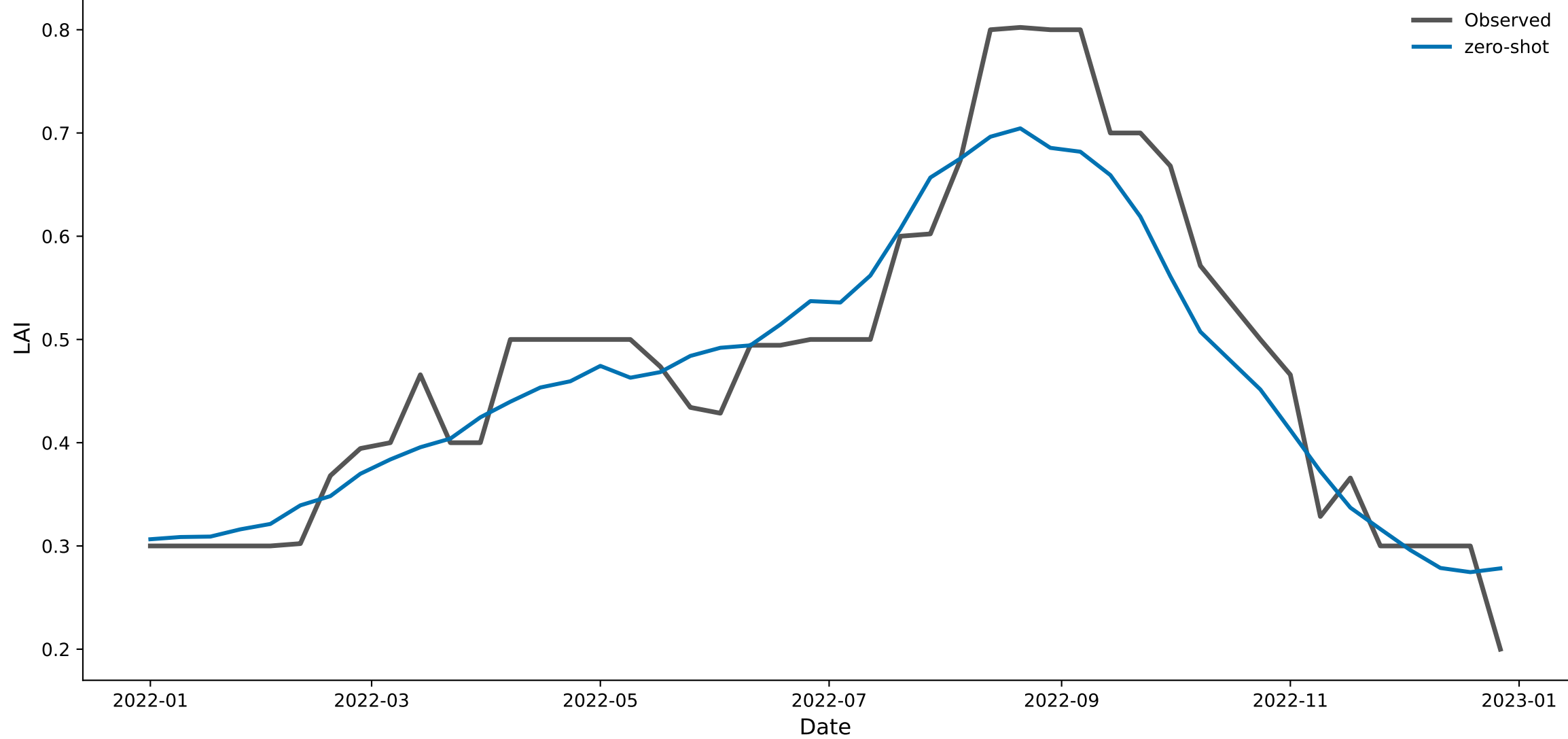
px050_shrubs_ne — Chronos-2 (zero-shot) predicted vs. observed LAI, 2022
