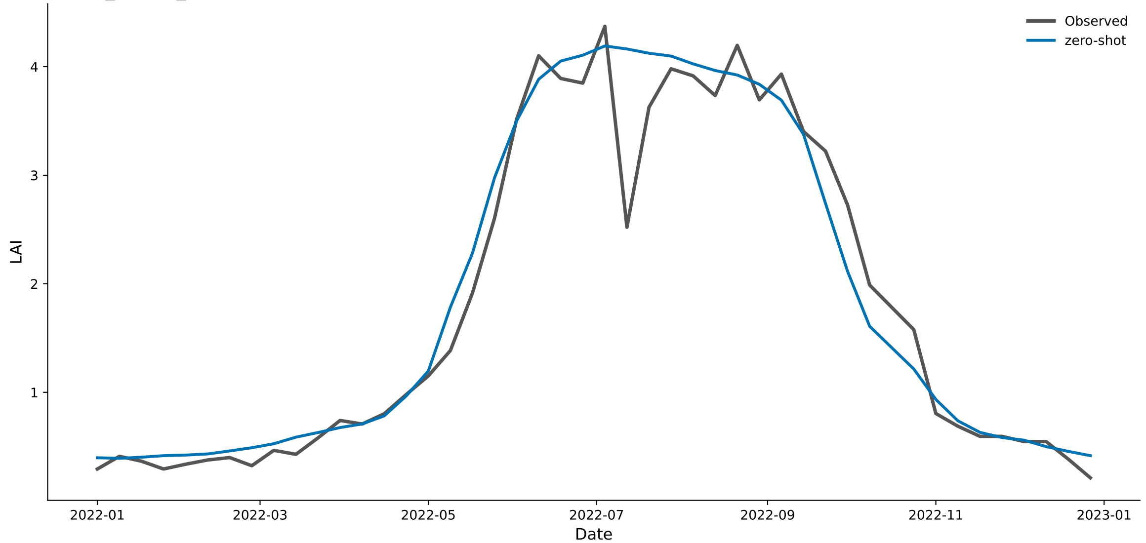
px052_shrubs_bd — Chronos-2 (zero-shot) predicted vs. observed LAI, 2022
