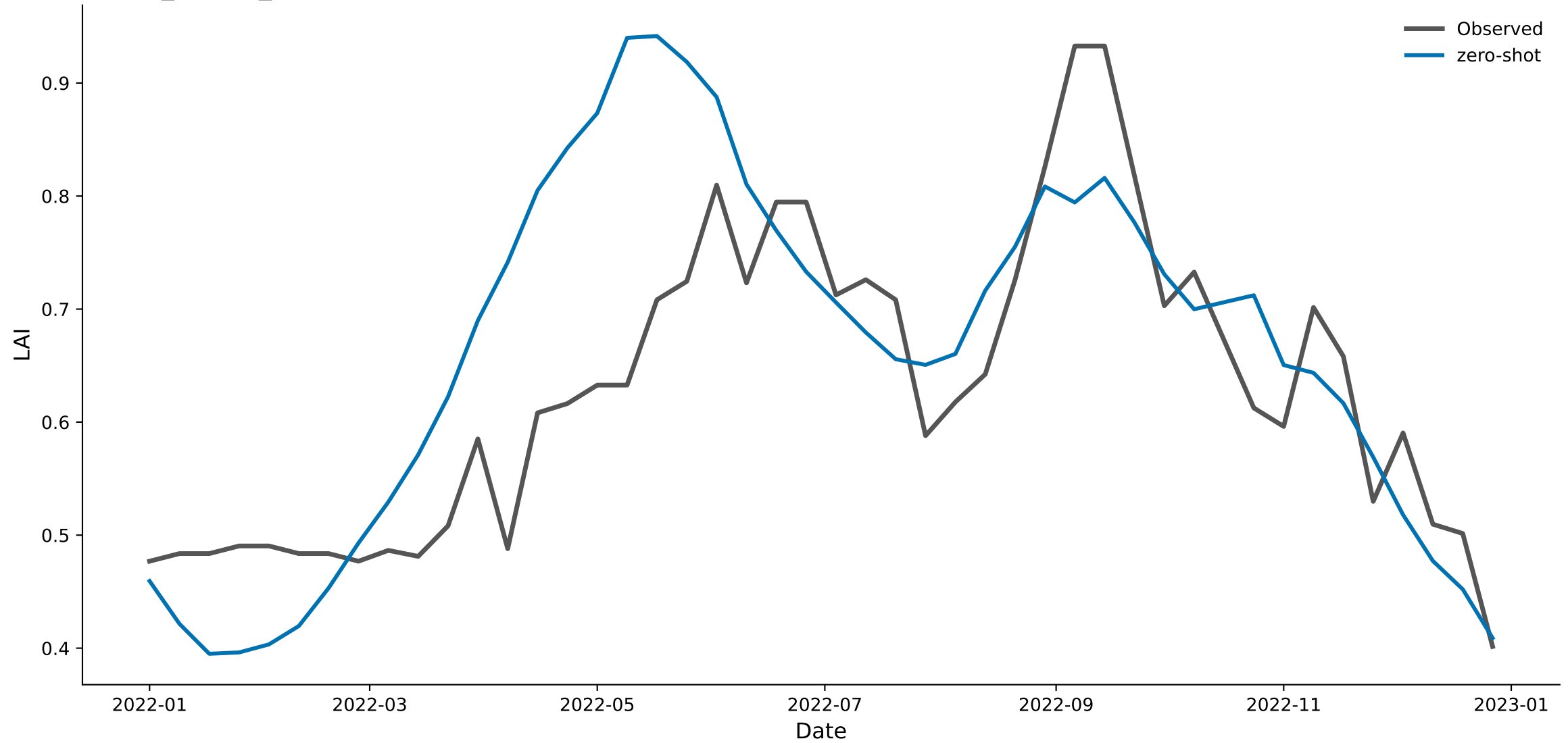
px059_shrubs_bd — Chronos-2 (zero-shot) predicted vs. observed LAI, 2022
