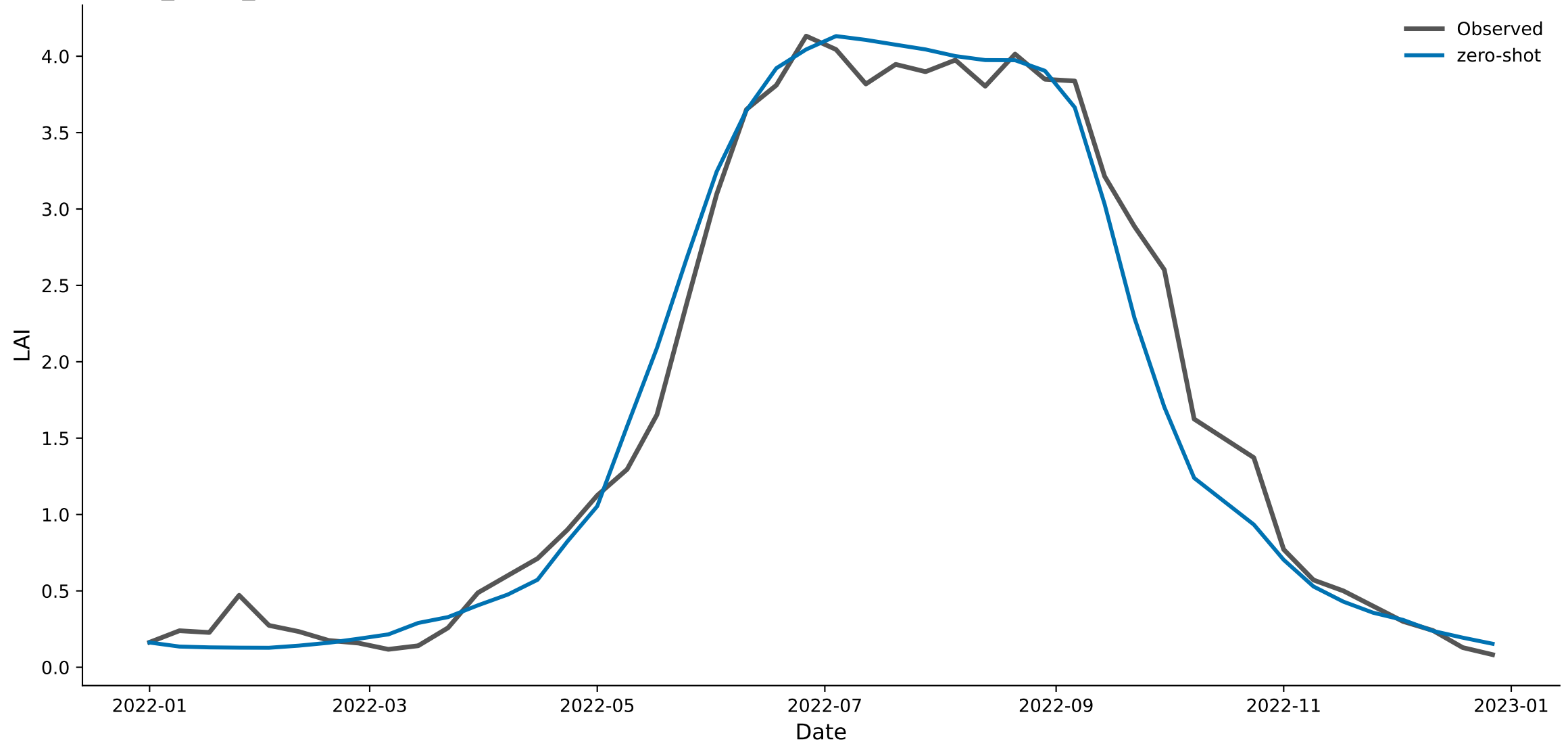
px060_grass_nat — Chronos-2 (zero-shot) predicted vs. observed LAI, 2022
