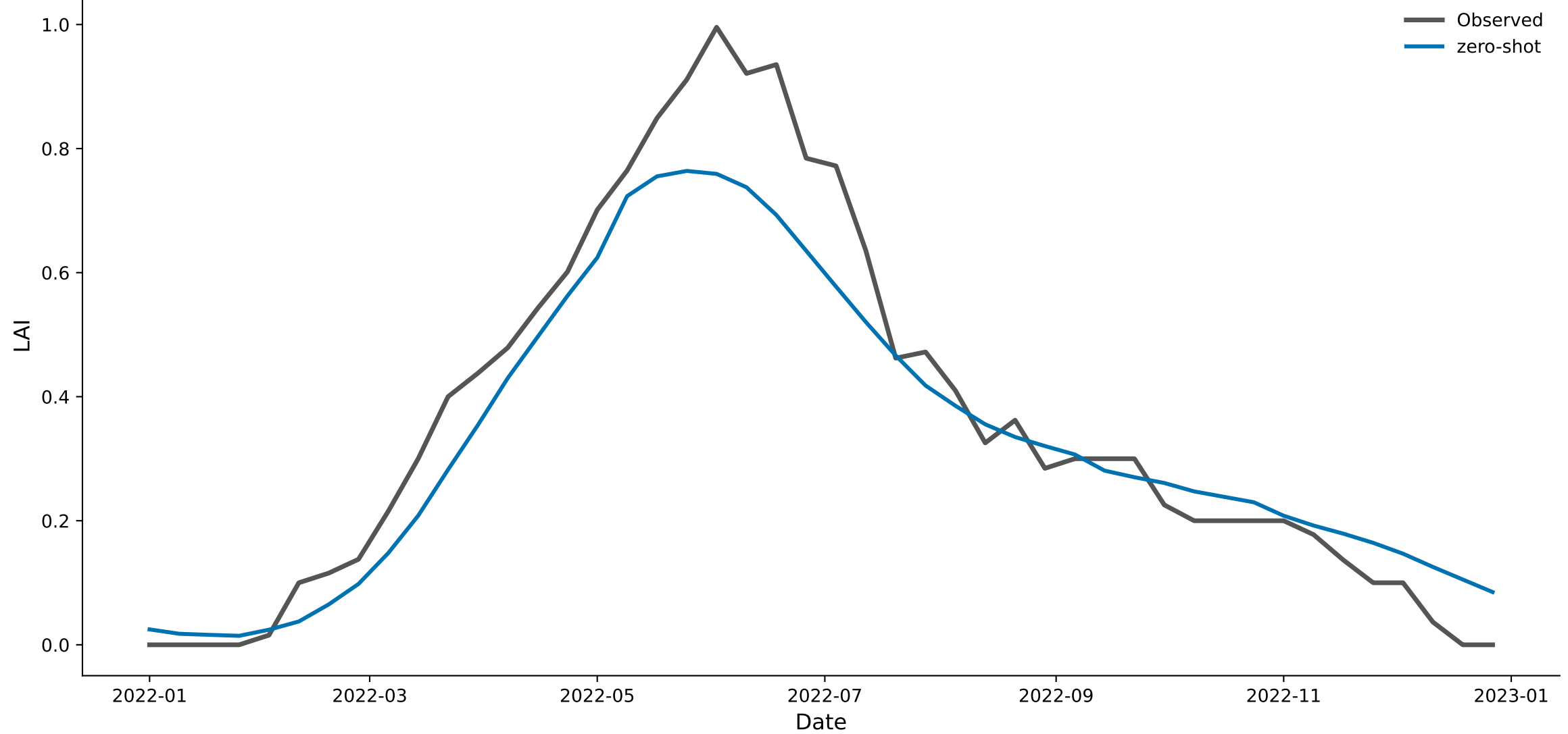
px061_grass_nat — Chronos-2 (zero-shot) predicted vs. observed LAI, 2022
