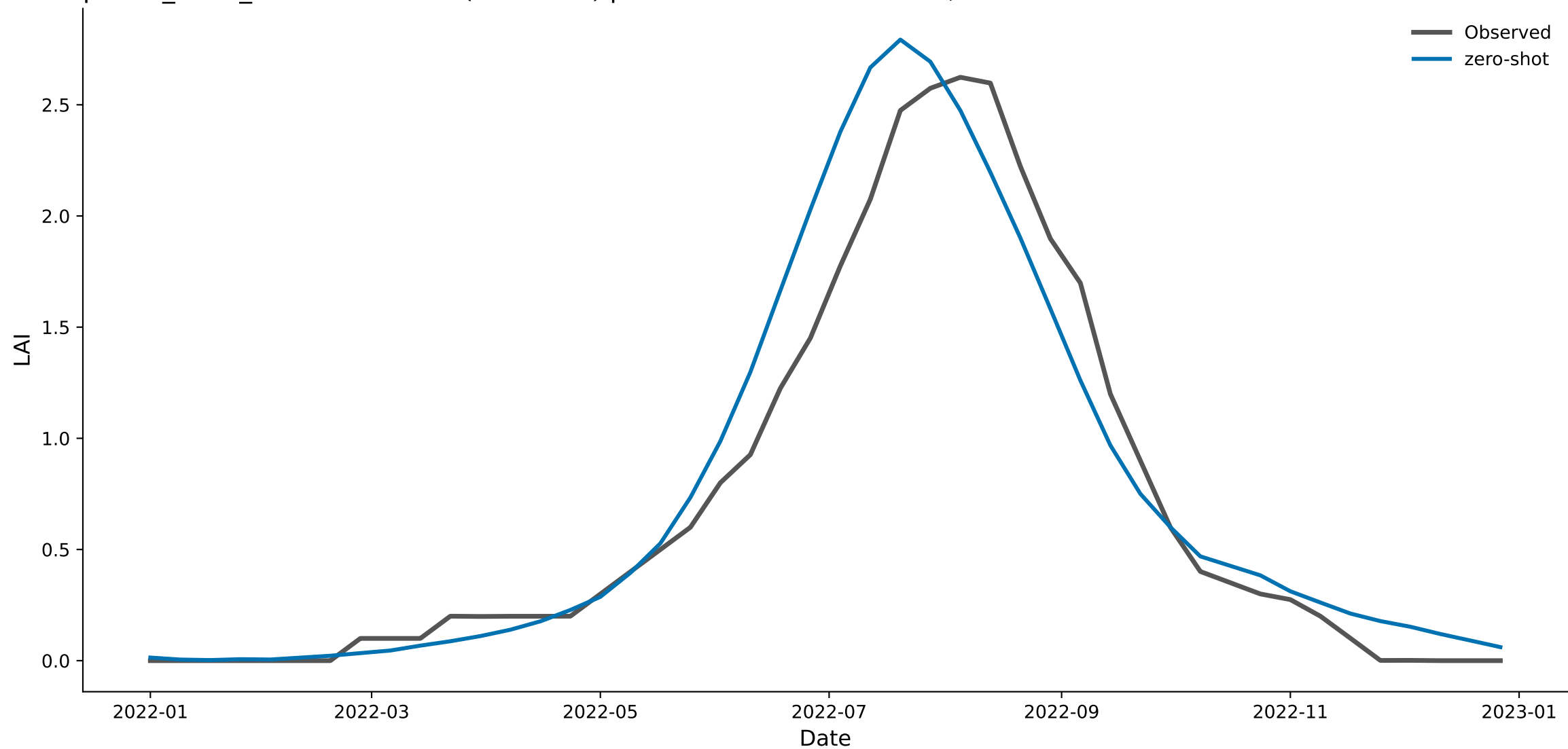
px069_trees_bd — Chronos-2 (zero-shot) predicted vs. observed LAI, 2022
