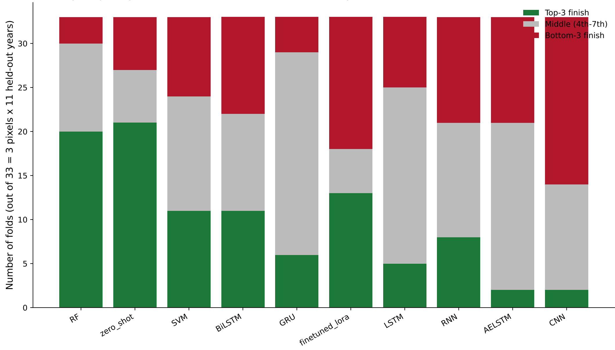
Ranking frequency across all 33 LOYO-CV folds, ordered by mean rank (best to worst)
