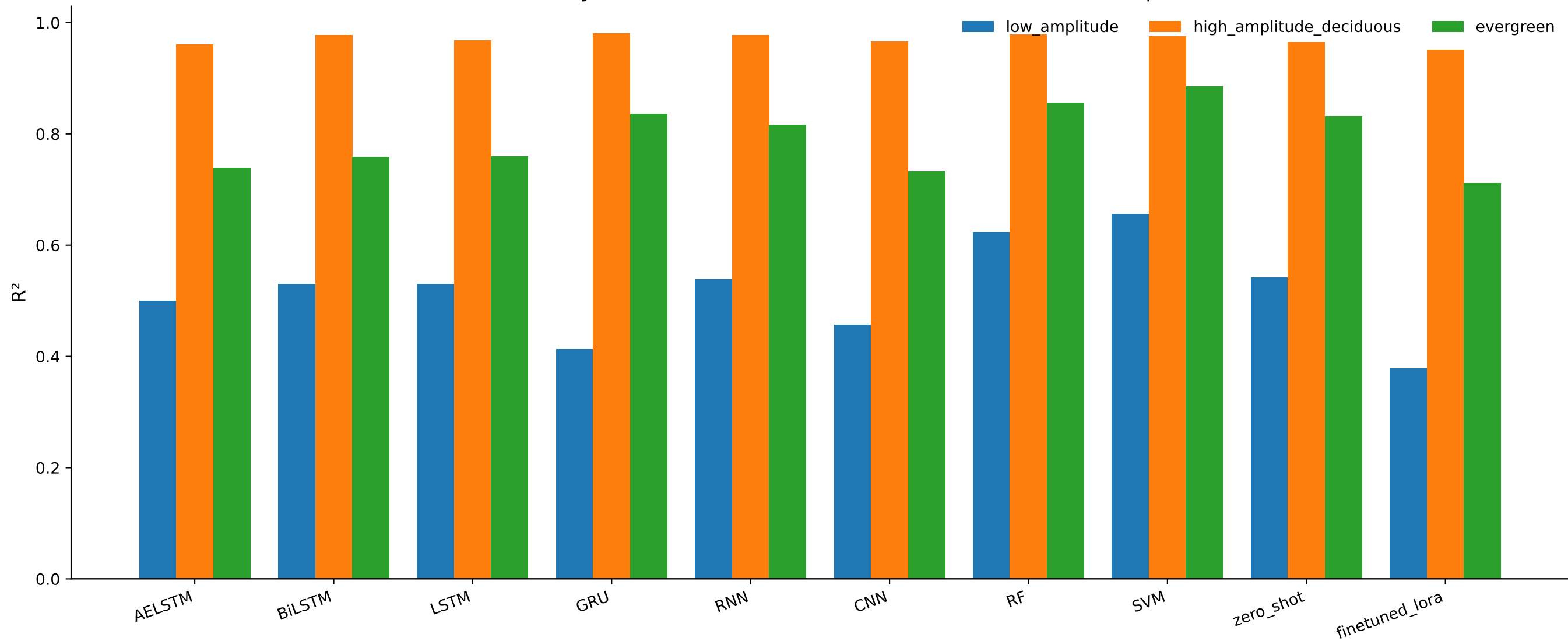
AELSTM-family models + Chronos-2 (zero-shot / LoRA): R^2 across pixels
