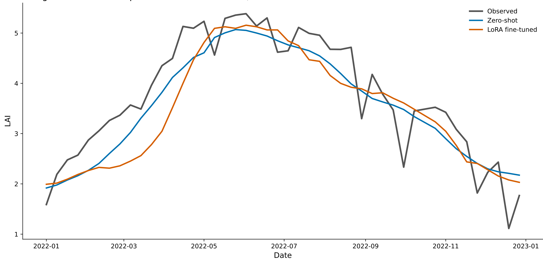
evergreen — Chronos-2 predicted vs. observed LAI, 2022
