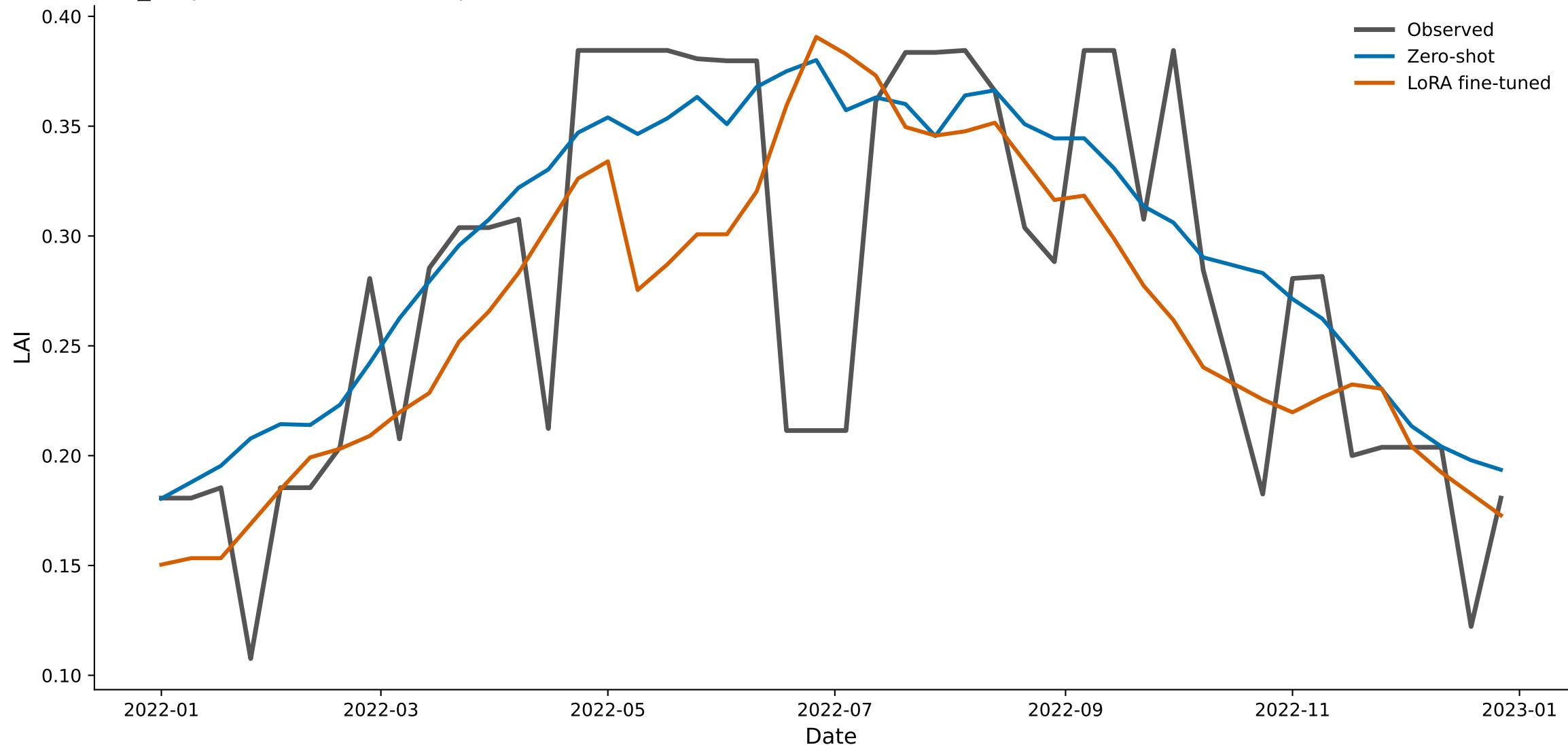
low_amplitude — Chronos-2 predicted vs. observed LAI, 2022
