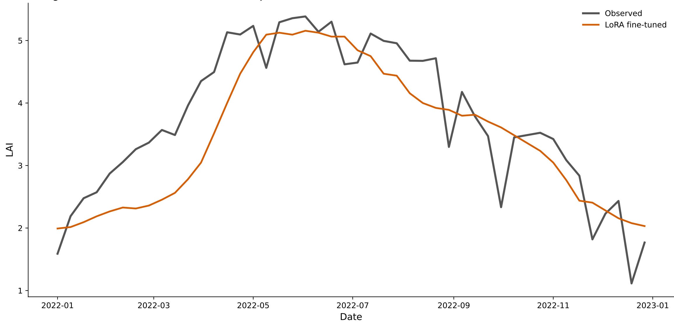
evergreen — Chronos-2 (LoRA fine-tuned) predicted vs. observed LAI, 2022
