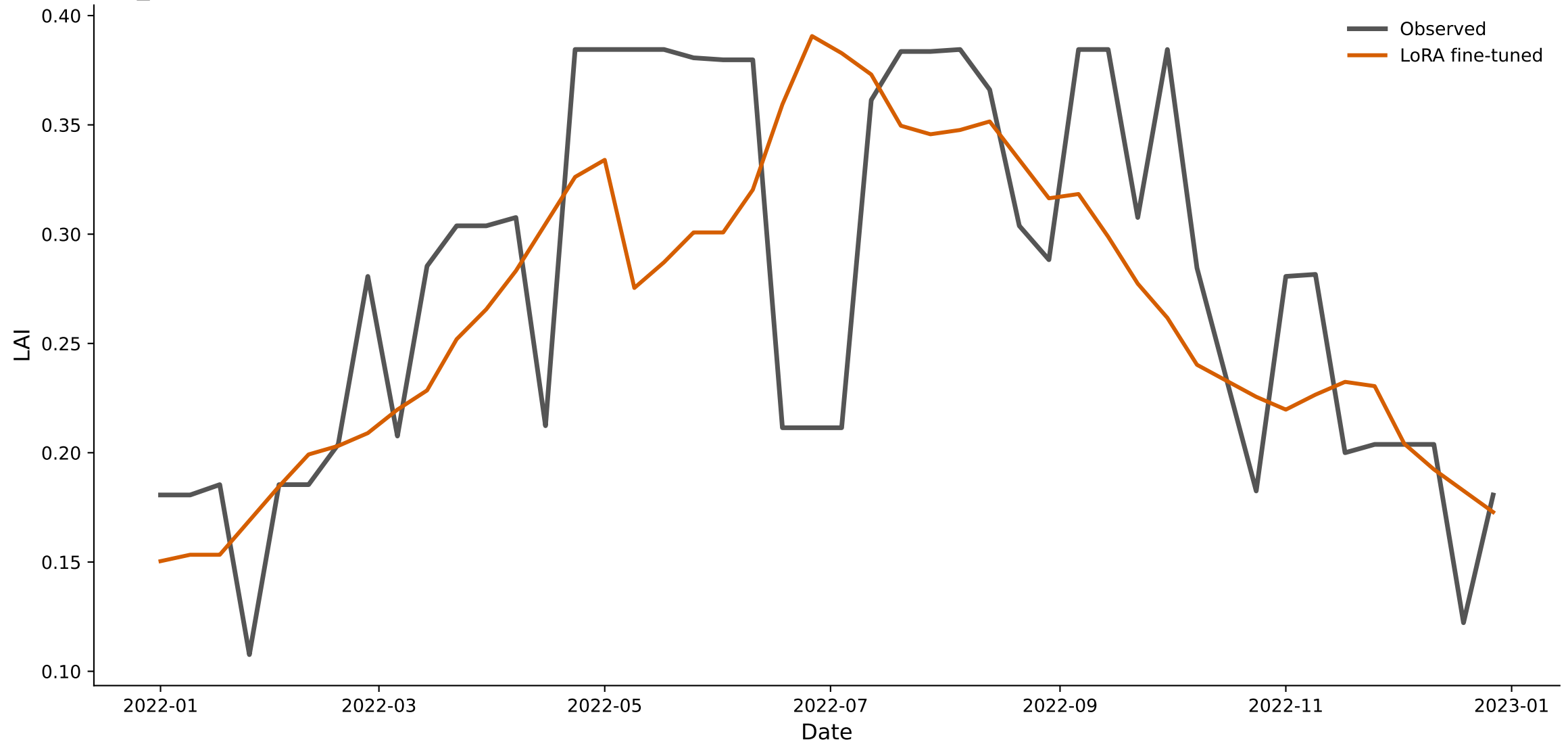
low_amplitude — Chronos-2 (LoRA fine-tuned) predicted vs. observed LAI, 2022
