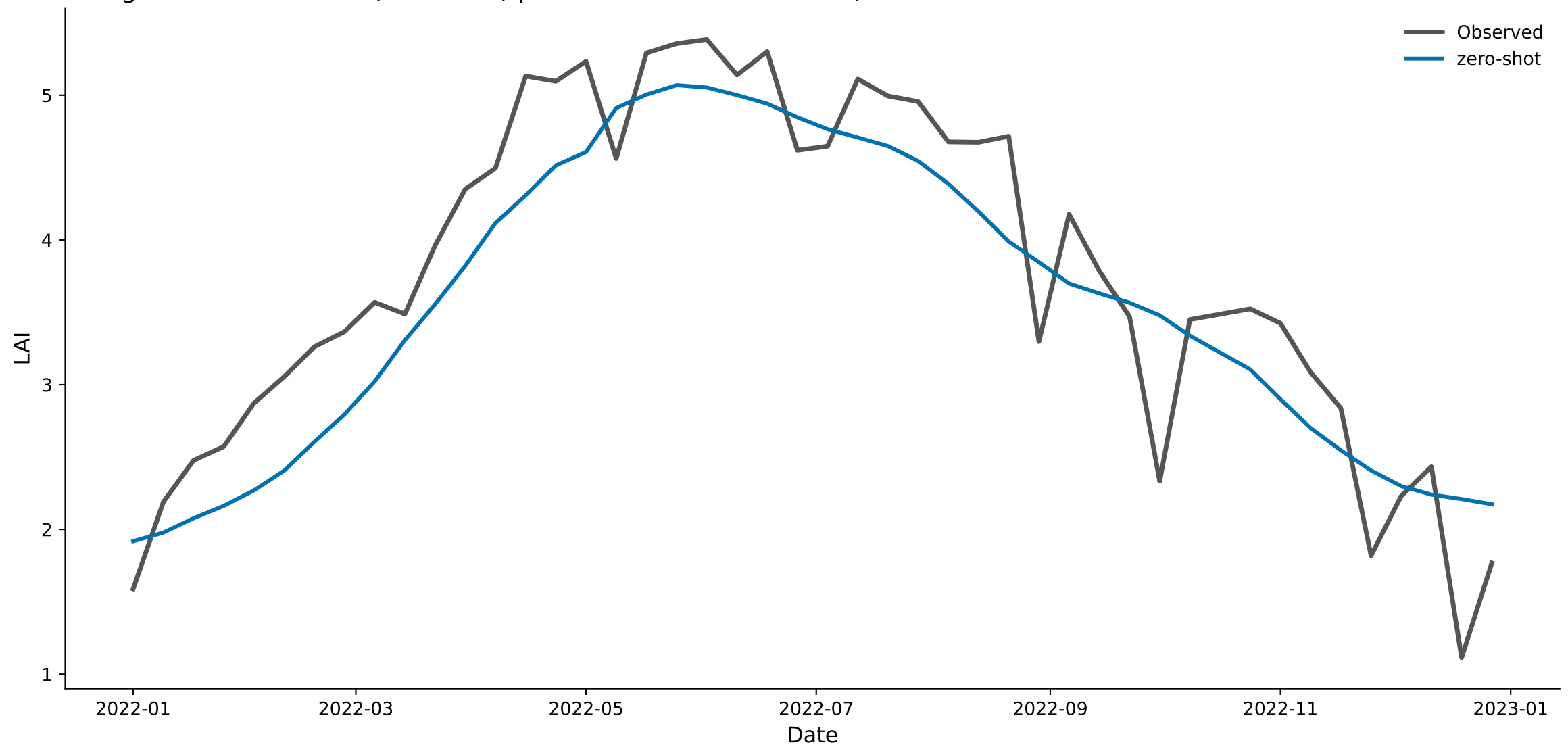
evergreen — Chronos-2 (zero-shot) predicted vs. observed LAI, 2022
