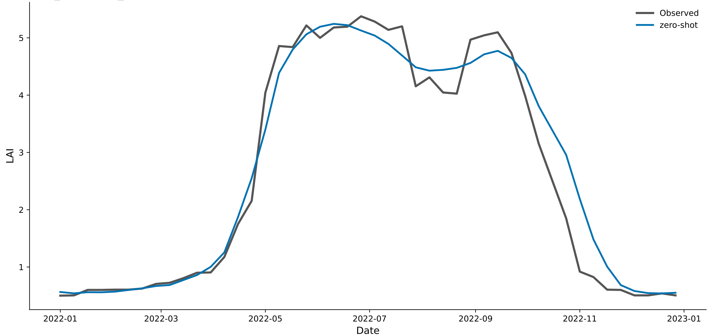
high_amplitude_deciduous — Chronos-2 (zero-shot) predicted vs. observed LAI, 2022
