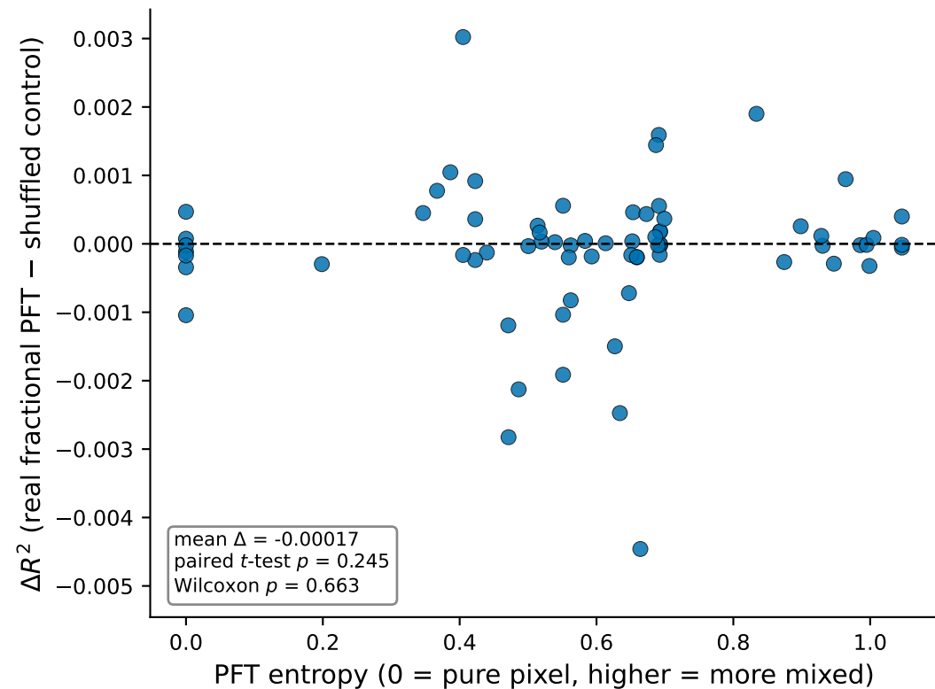
(a) Real vs. shuffled PFT, per pixel ( n = 70 )
