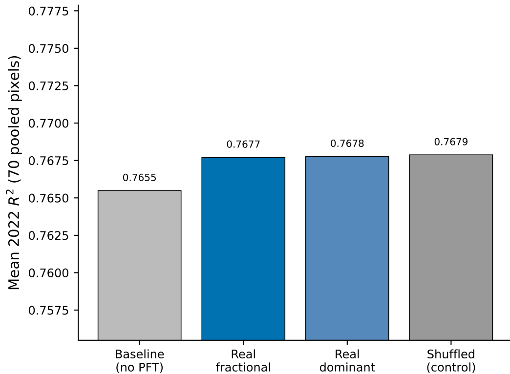
(b) Mean R^2 : real vs. shuffled PFT
