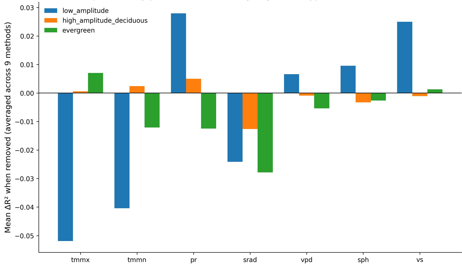
Predictor importance by pixel — does it shift by vegetation type?
