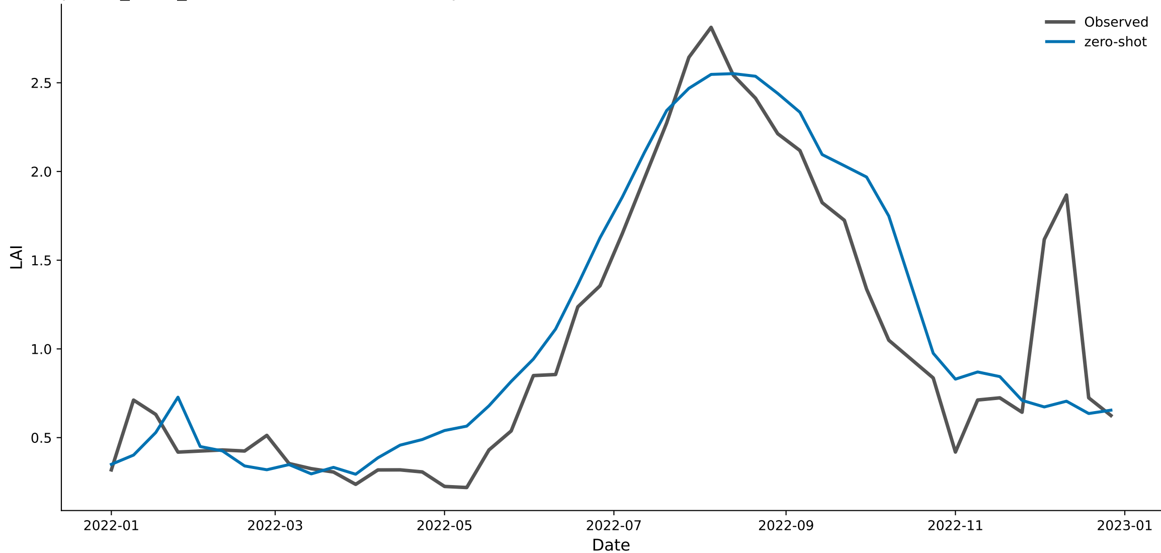
px004_trees_ne — Chronos-2 (zero-shot) predicted vs. observed LAI, 2022
