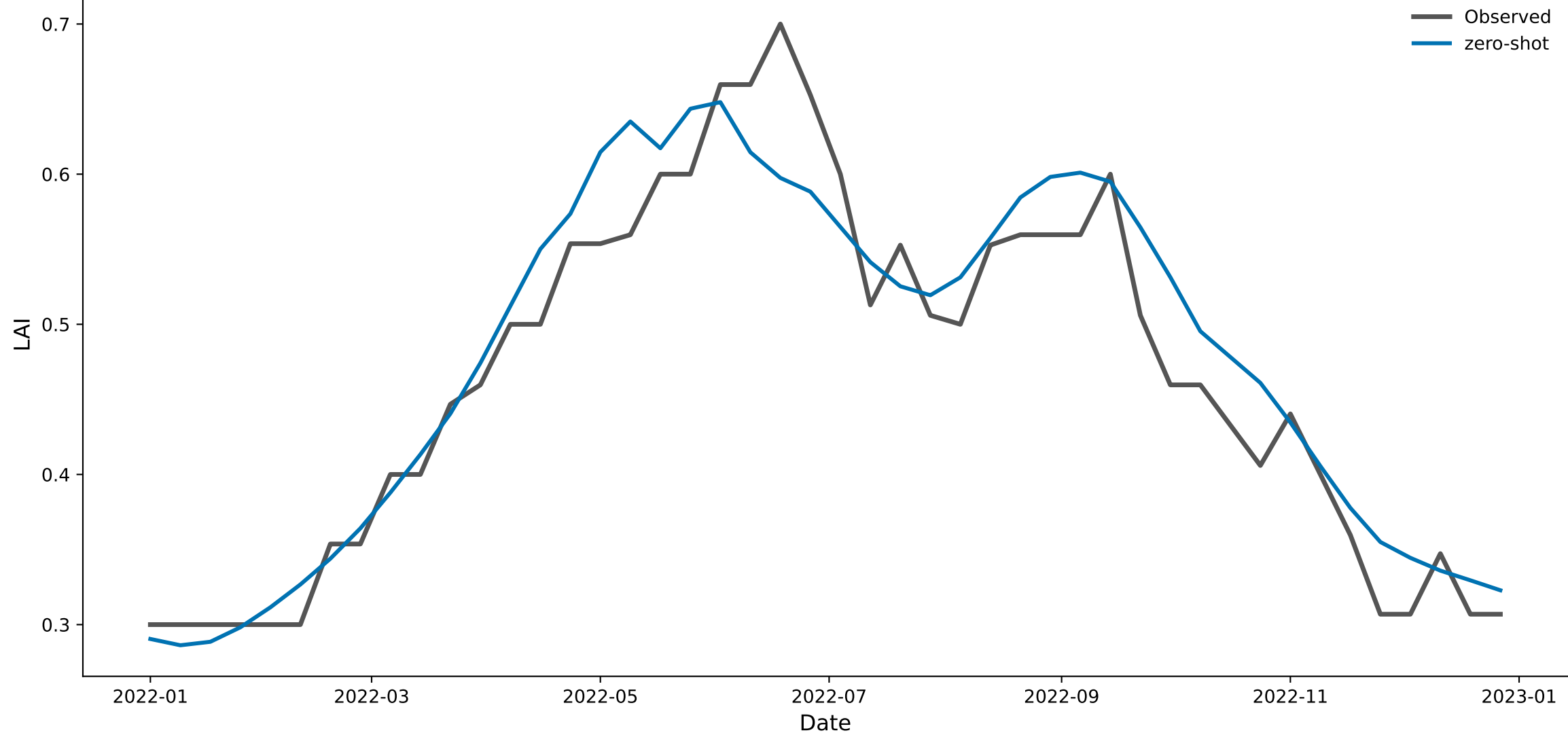
px007_shrubs_ne — Chronos-2 (zero-shot) predicted vs. observed LAI, 2022
