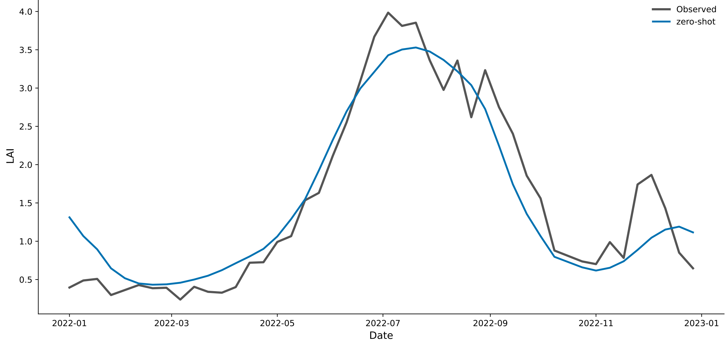
px010_grass_nat — Chronos-2 (zero-shot) predicted vs. observed LAI, 2022
