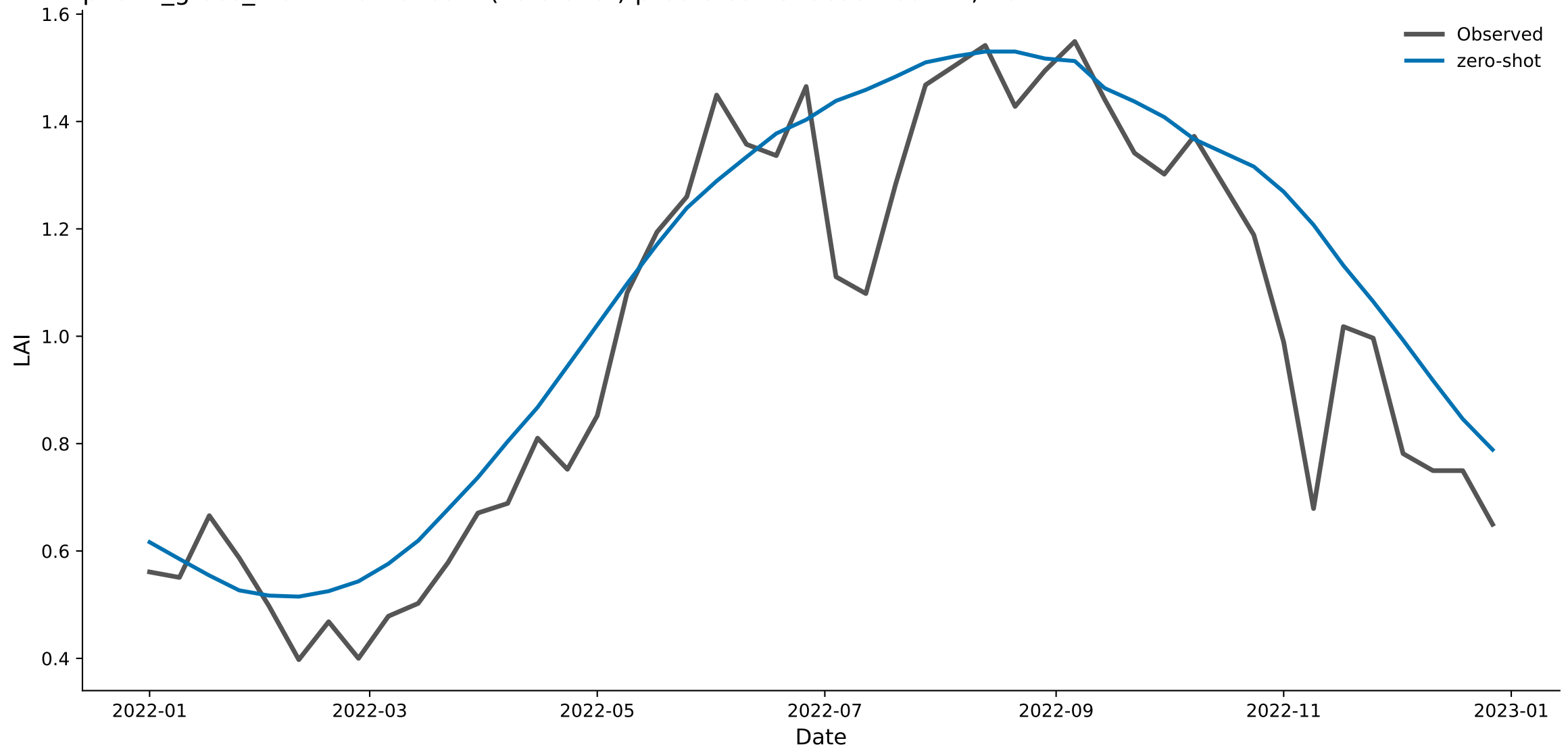
px027_grass_man — Chronos-2 (zero-shot) predicted vs. observed LAI, 2022
