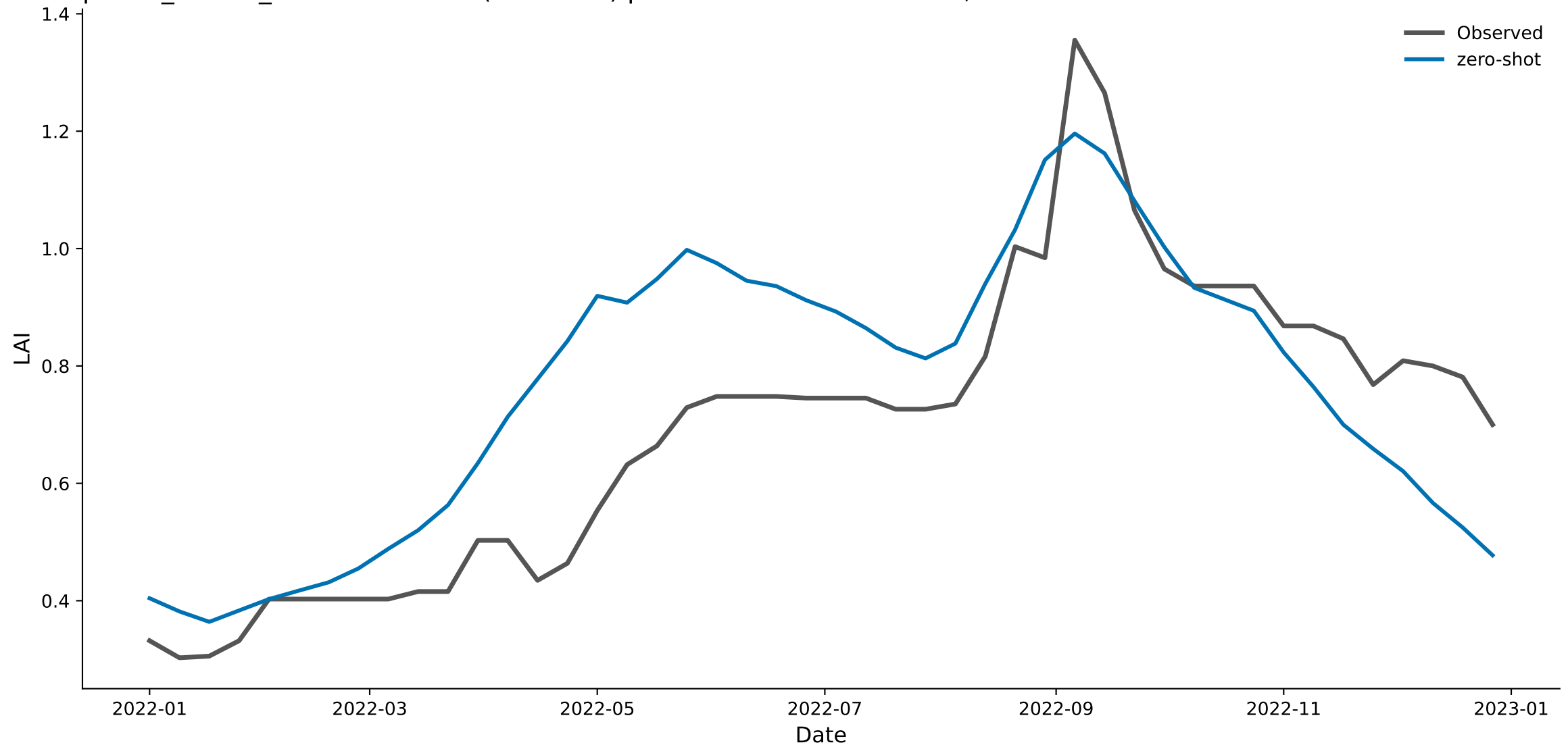
px035_shrubs_nd — Chronos-2 (zero-shot) predicted vs. observed LAI, 2022
