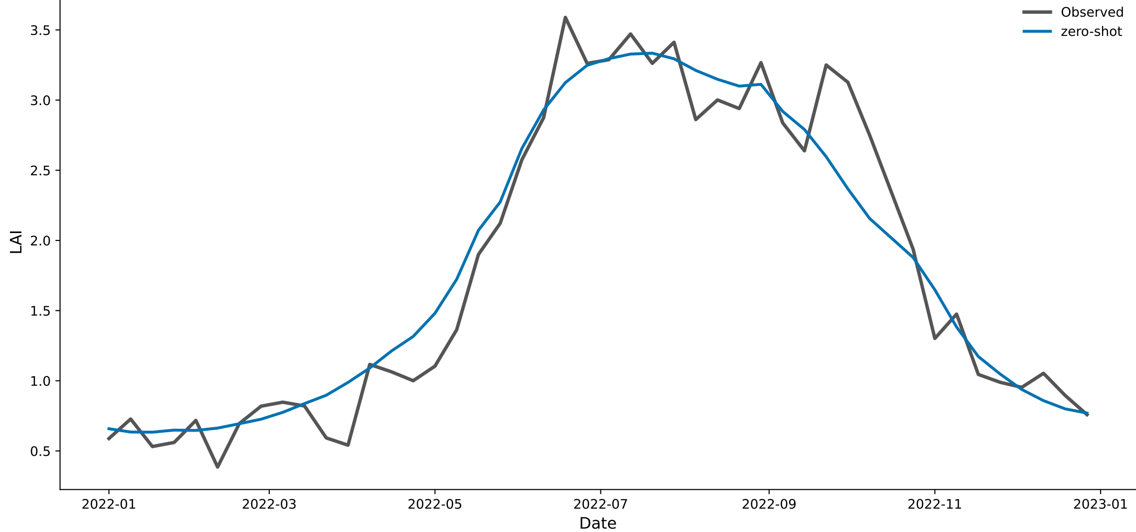
px039_trees_ne — Chronos-2 (zero-shot) predicted vs. observed LAI, 2022
