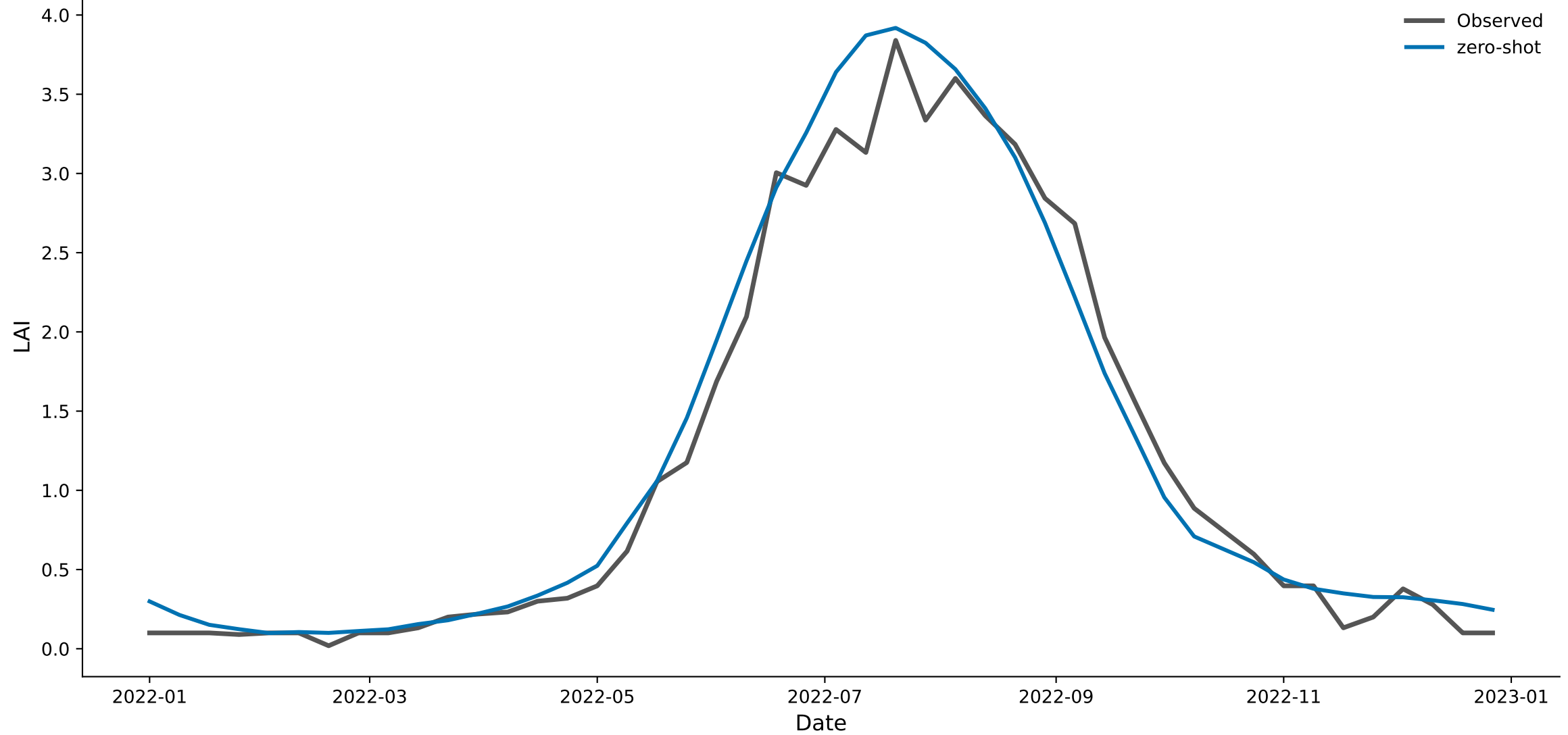
px043_grass_nat — Chronos-2 (zero-shot) predicted vs. observed LAI, 2022
