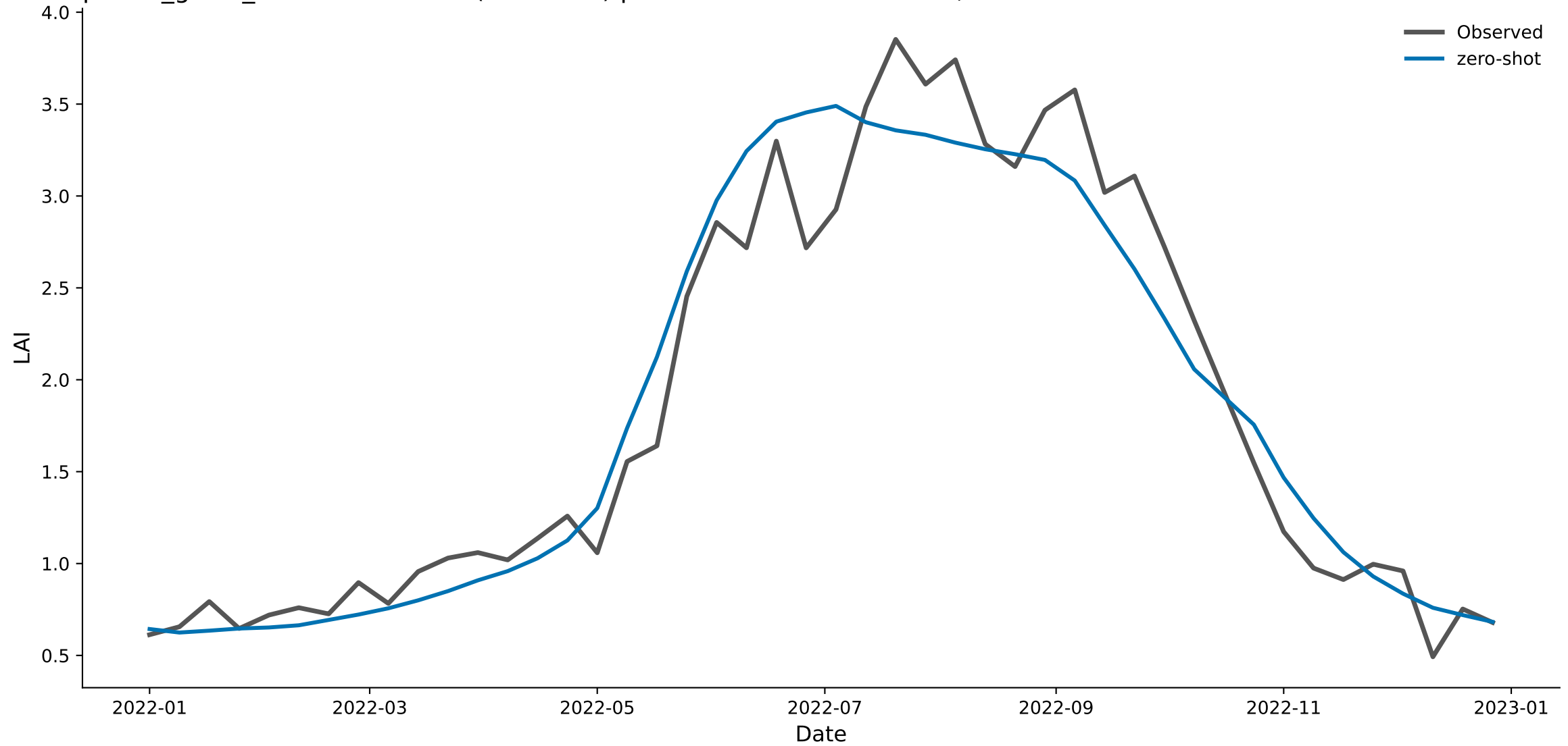
px044_grass_nat — Chronos-2 (zero-shot) predicted vs. observed LAI, 2022
