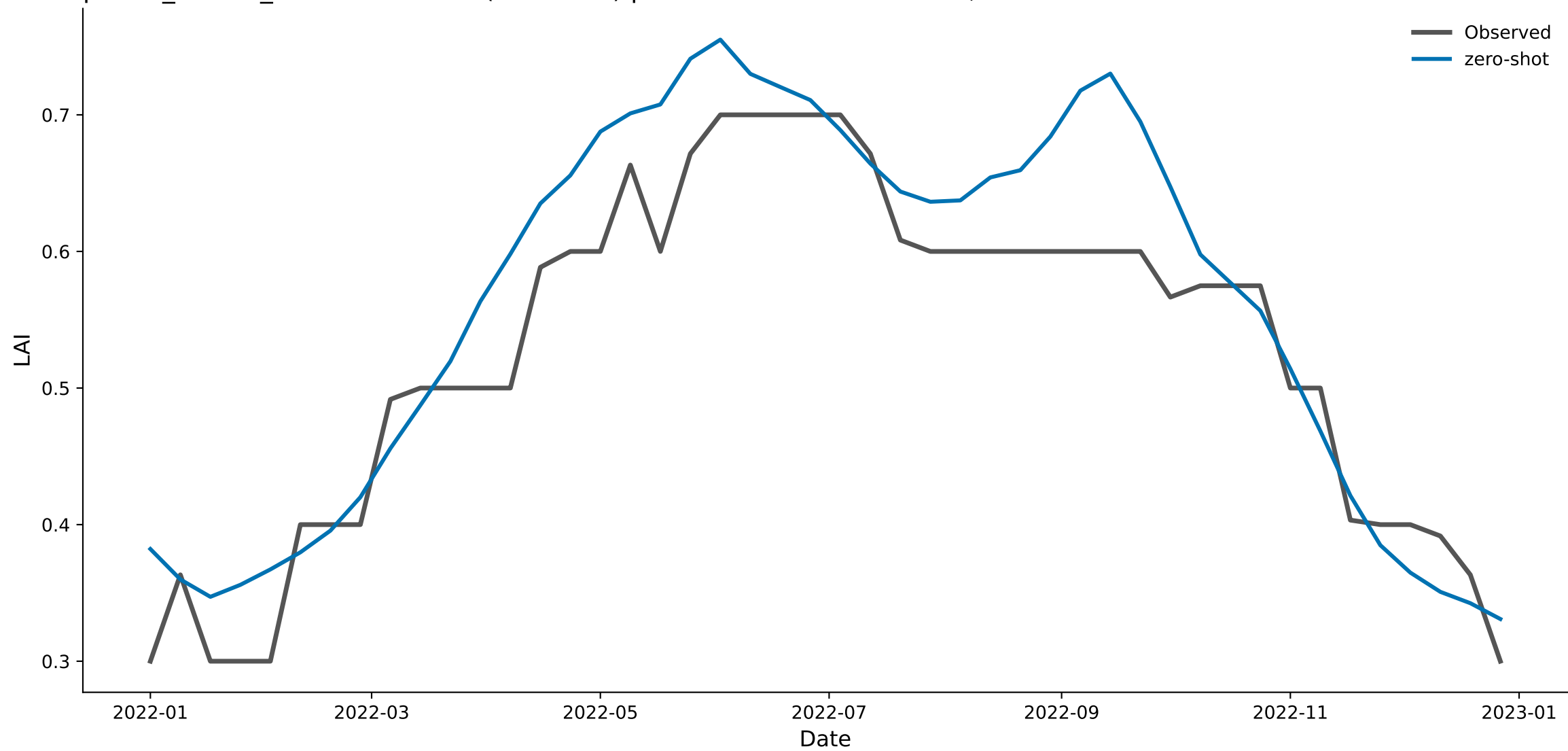
px055_shrubs_bd — Chronos-2 (zero-shot) predicted vs. observed LAI, 2022
