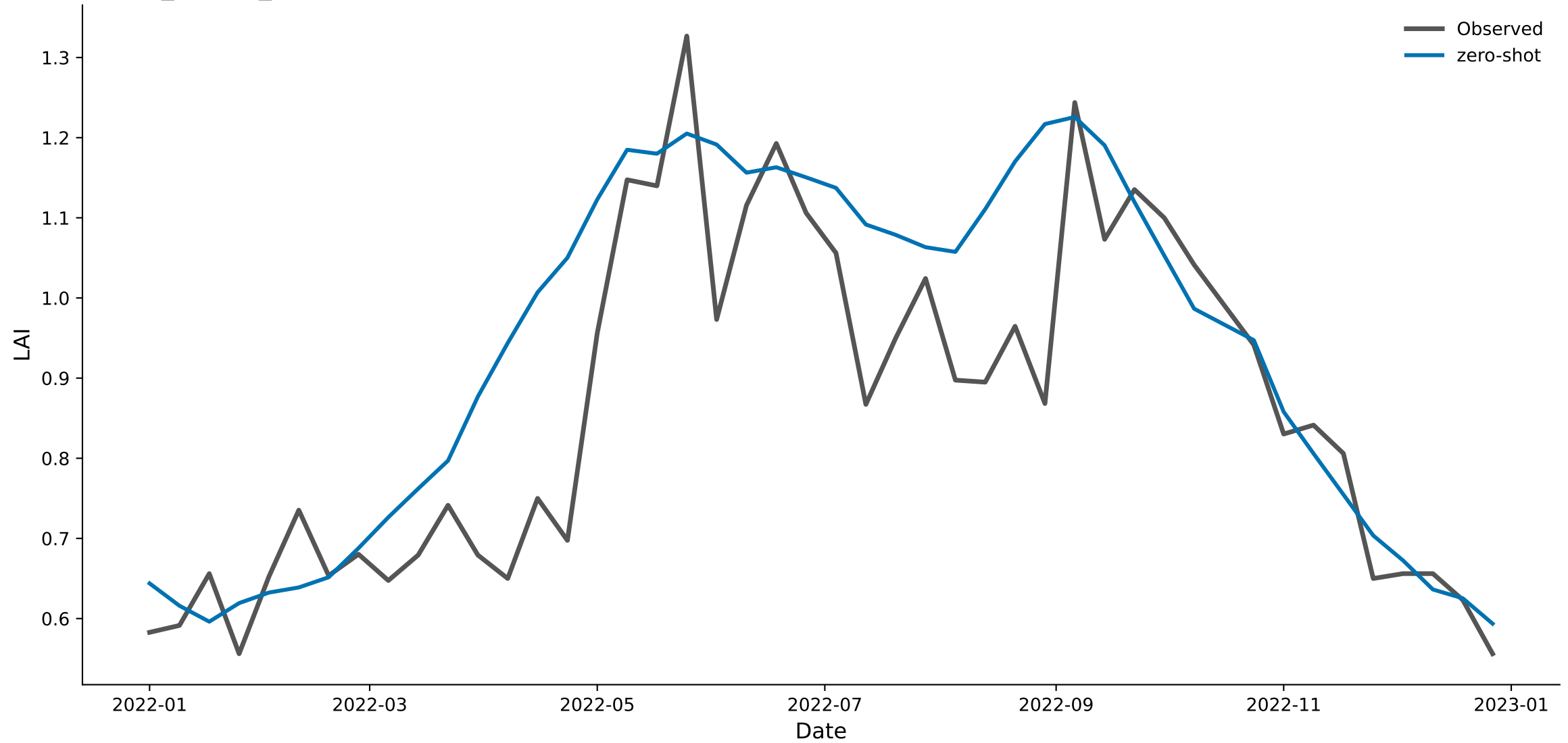
px064_shrubs_bd — Chronos-2 (zero-shot) predicted vs. observed LAI, 2022
