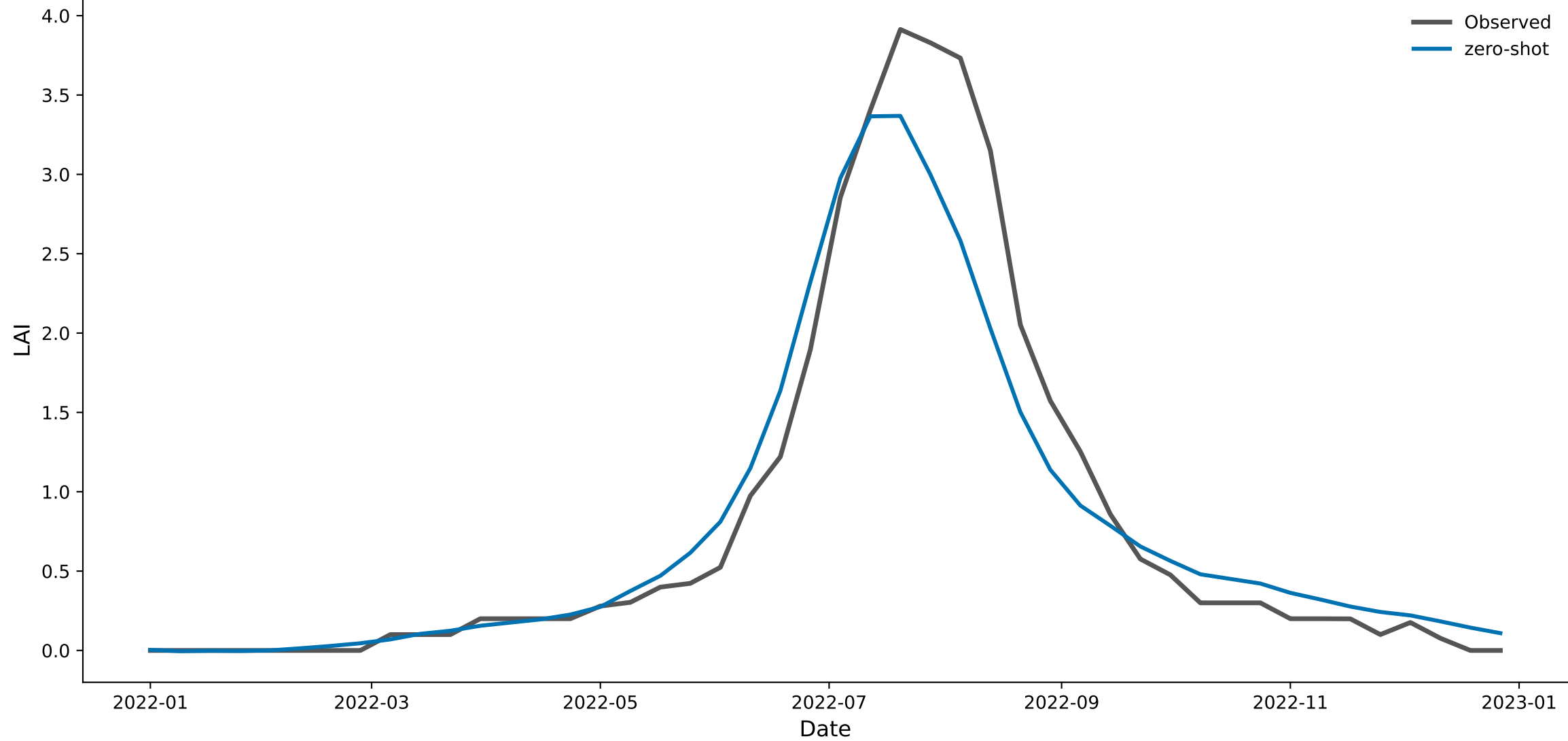
px067_grass_man — Chronos-2 (zero-shot) predicted vs. observed LAI, 2022
