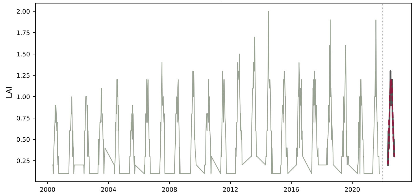
g019_trees_bd — Canada deciduous broadleaf forest R^2=0.637 , Pearson r=0.811 , context=626 steps
