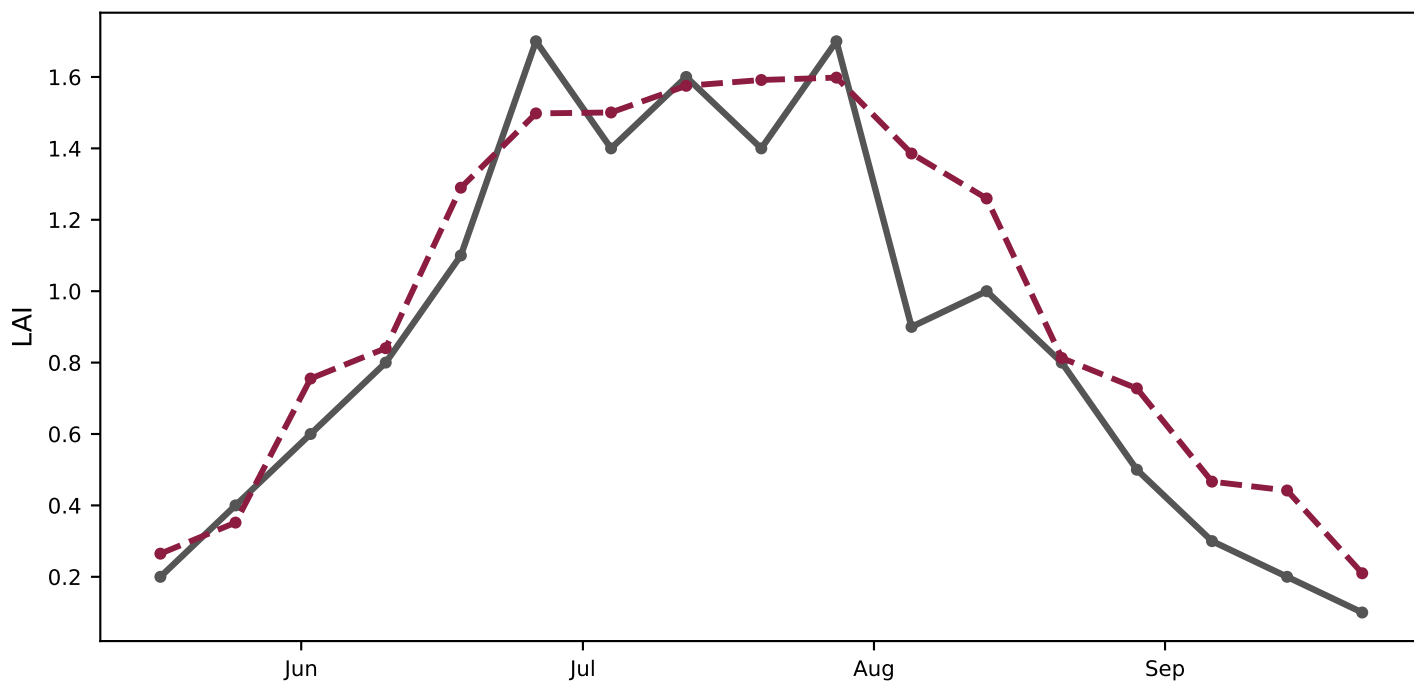
g014_trees_ne — Siberia / Boreal Eurasia evergreen forest R 2 =0.793, Pearson r=0.897
