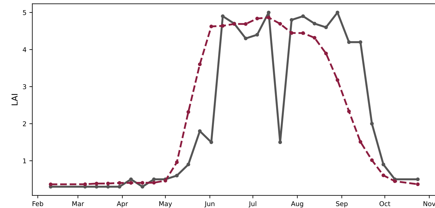
g068_grass_nat — Southern S. America grassland R 2 =0.708, Pearson r=0.855
