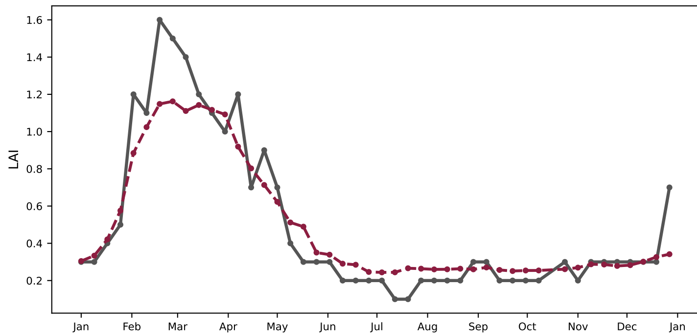
g009_grass_nat — Canada grassland R 2 =0.802, Pearson r=0.910
