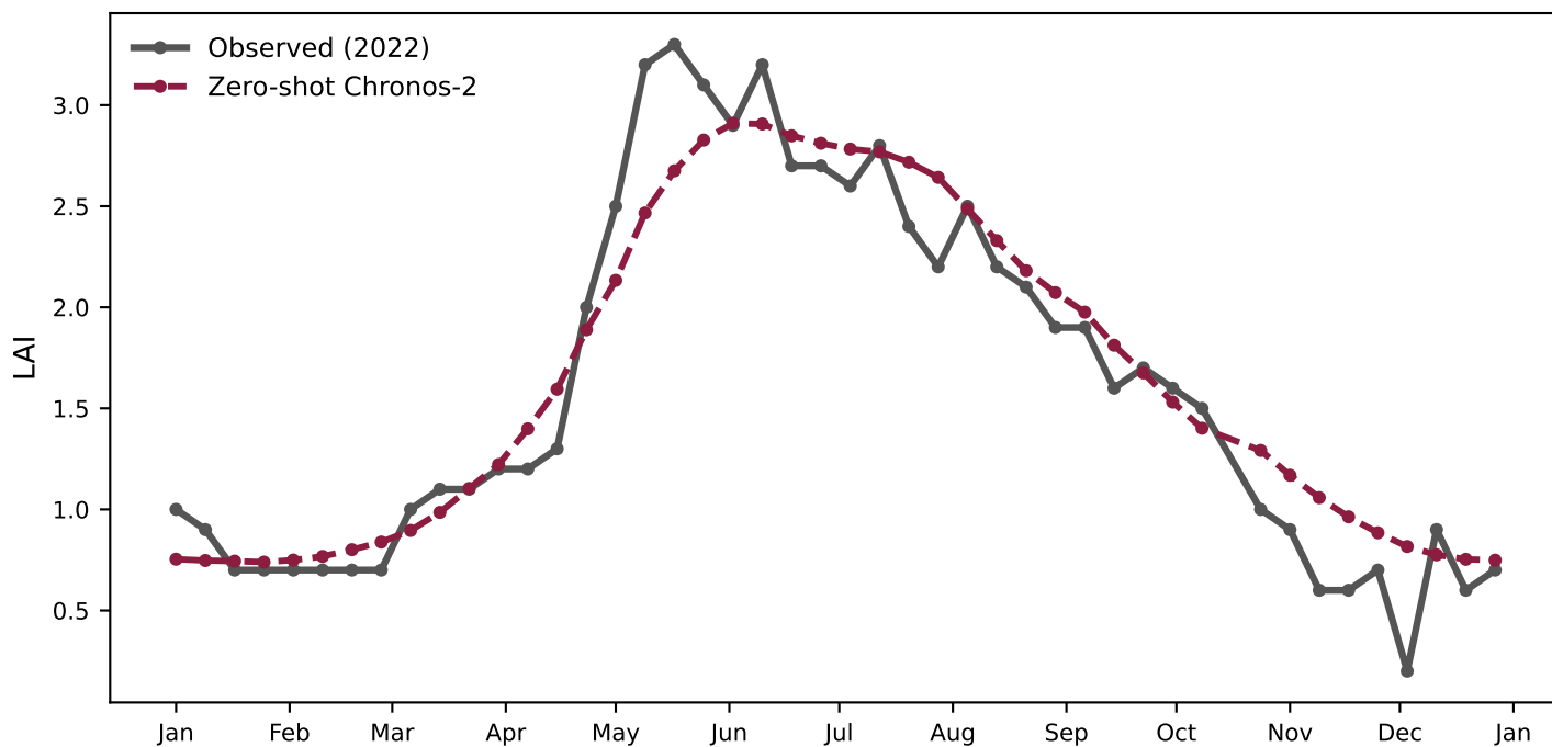
g005_grass_nat — Siberia / Boreal Eurasia grassland R 2 =0.871, Pearson r=0.956
