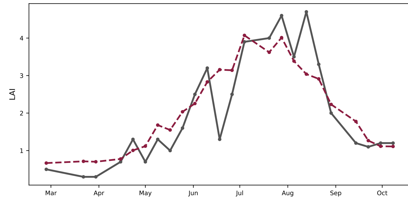
g035_grass_man — East Asia managed grassland R 2 =0.724, Pearson r=0.885
