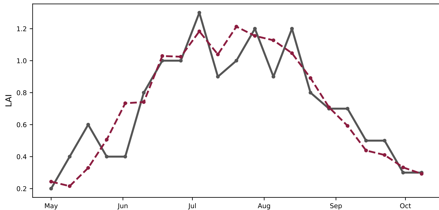
g019_trees_bd — Canada deciduous broadleaf forest R 2 =0.637, Pearson r=0.811
