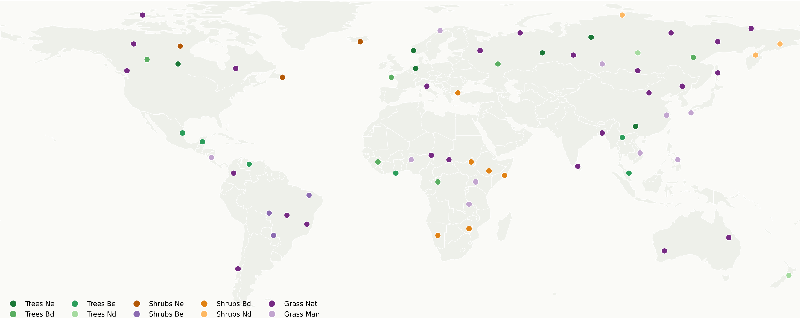
70 non-CONUS global pixels selected for the ERA5+MODIS zero-shot experiment (CONUS explicitly excluded by design; 68/70 had usable LAI)
