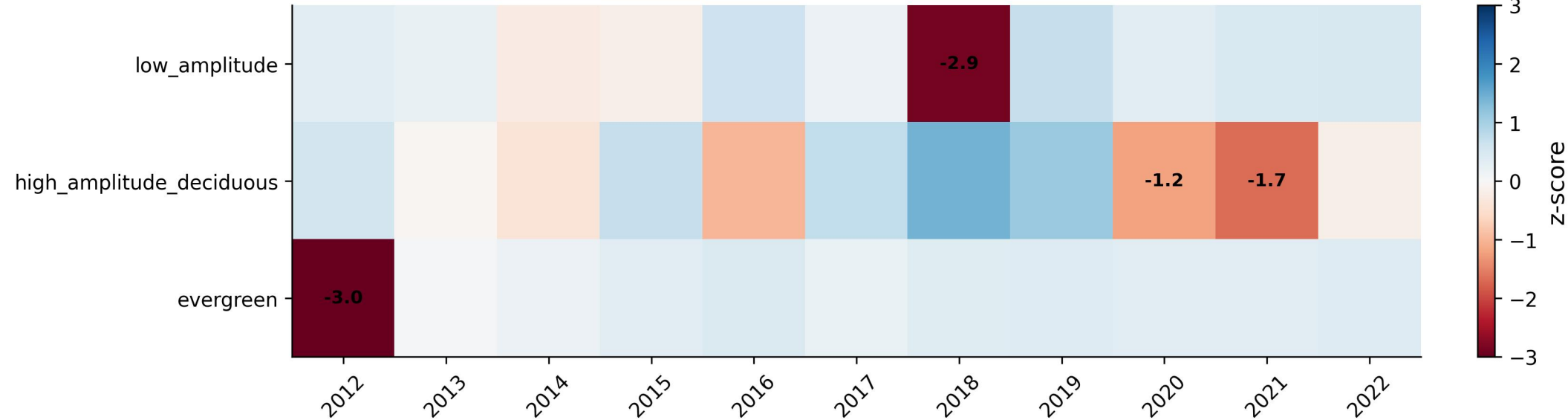
Year difficulty: z-score of median R^2 across all 10 models, within each pixel (red = harder than that pixel's typical year)
