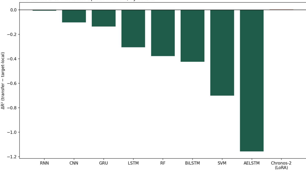
How much R^2 is lost under spatial transfer, by model
