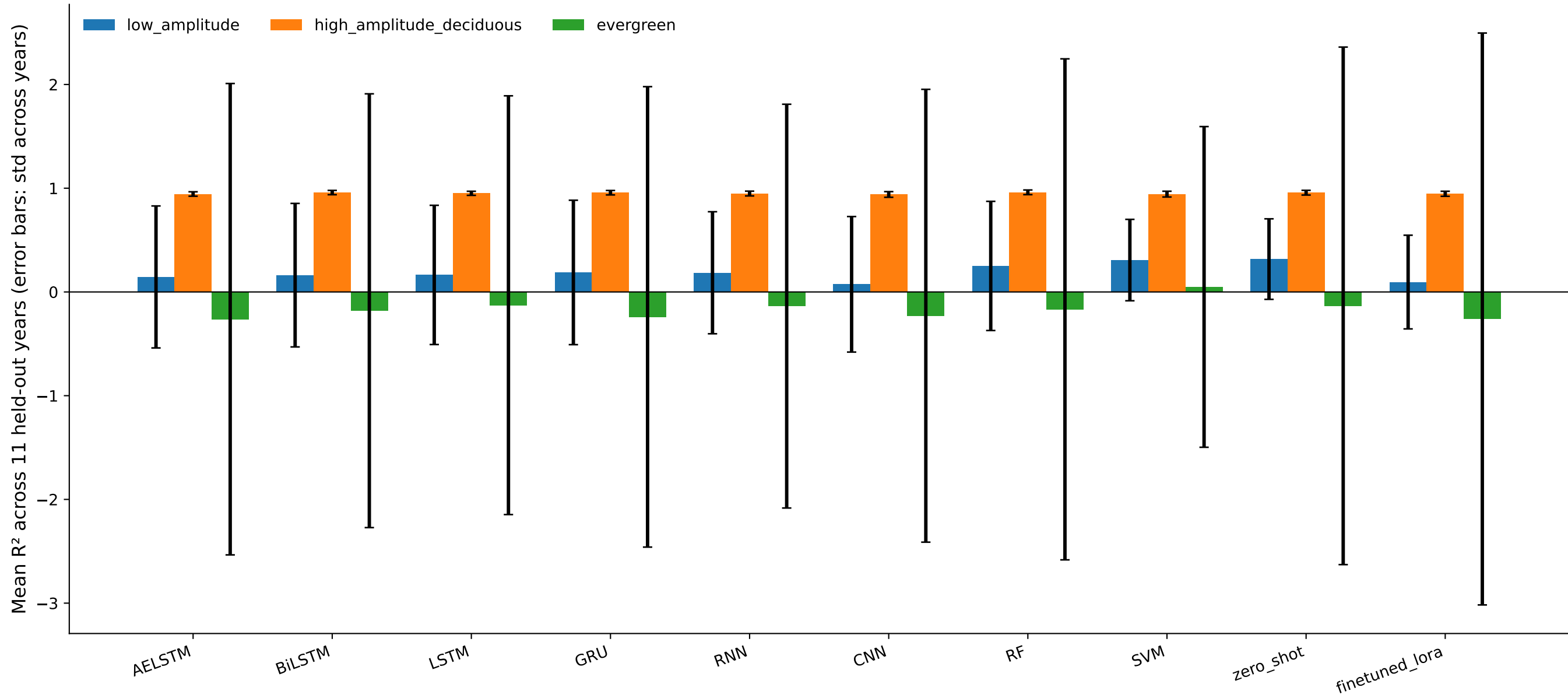
LOYO-CV: mean \pm std R^2 across held-out years, all 10 methods
