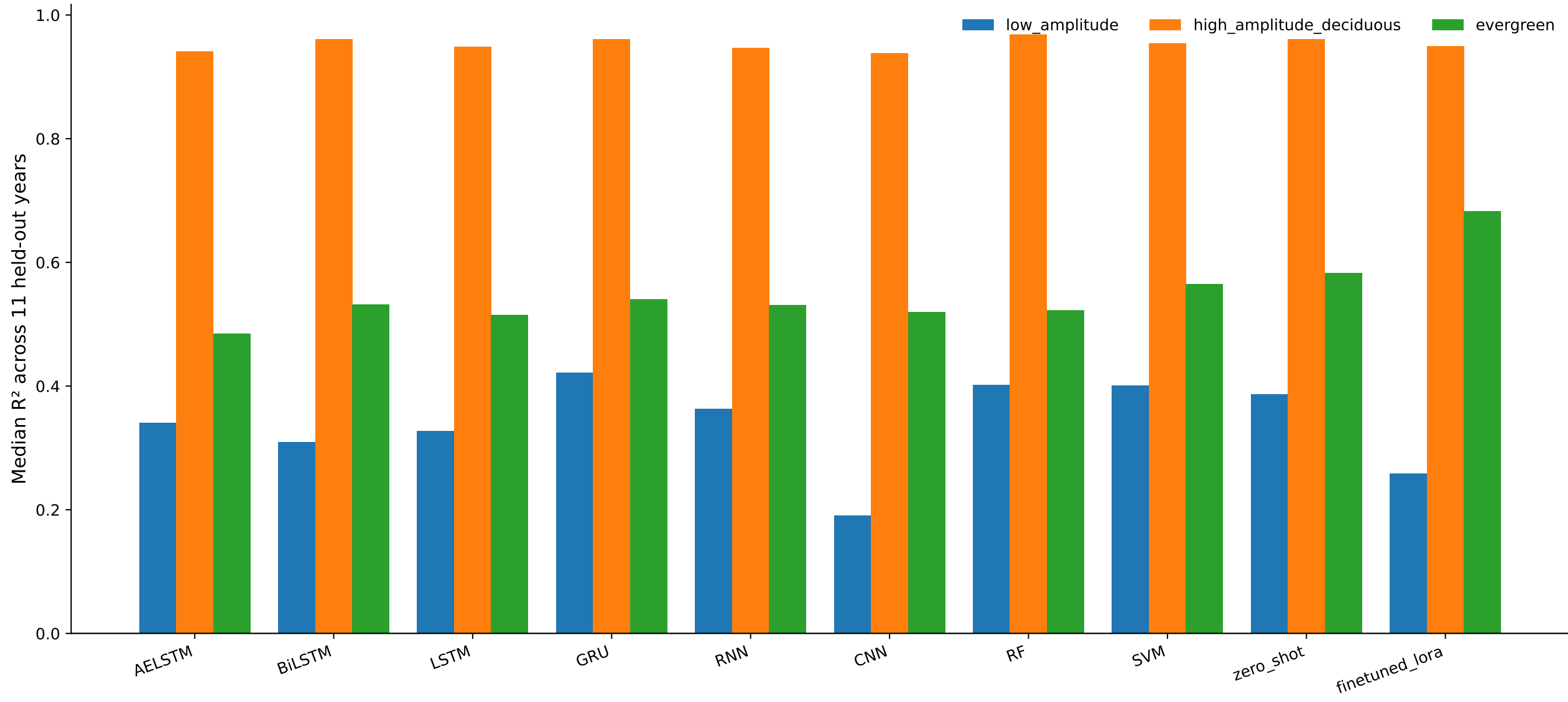
LOYO-CV: median R 2 across held-out years (robust to single-year outliers), all 10 methods
