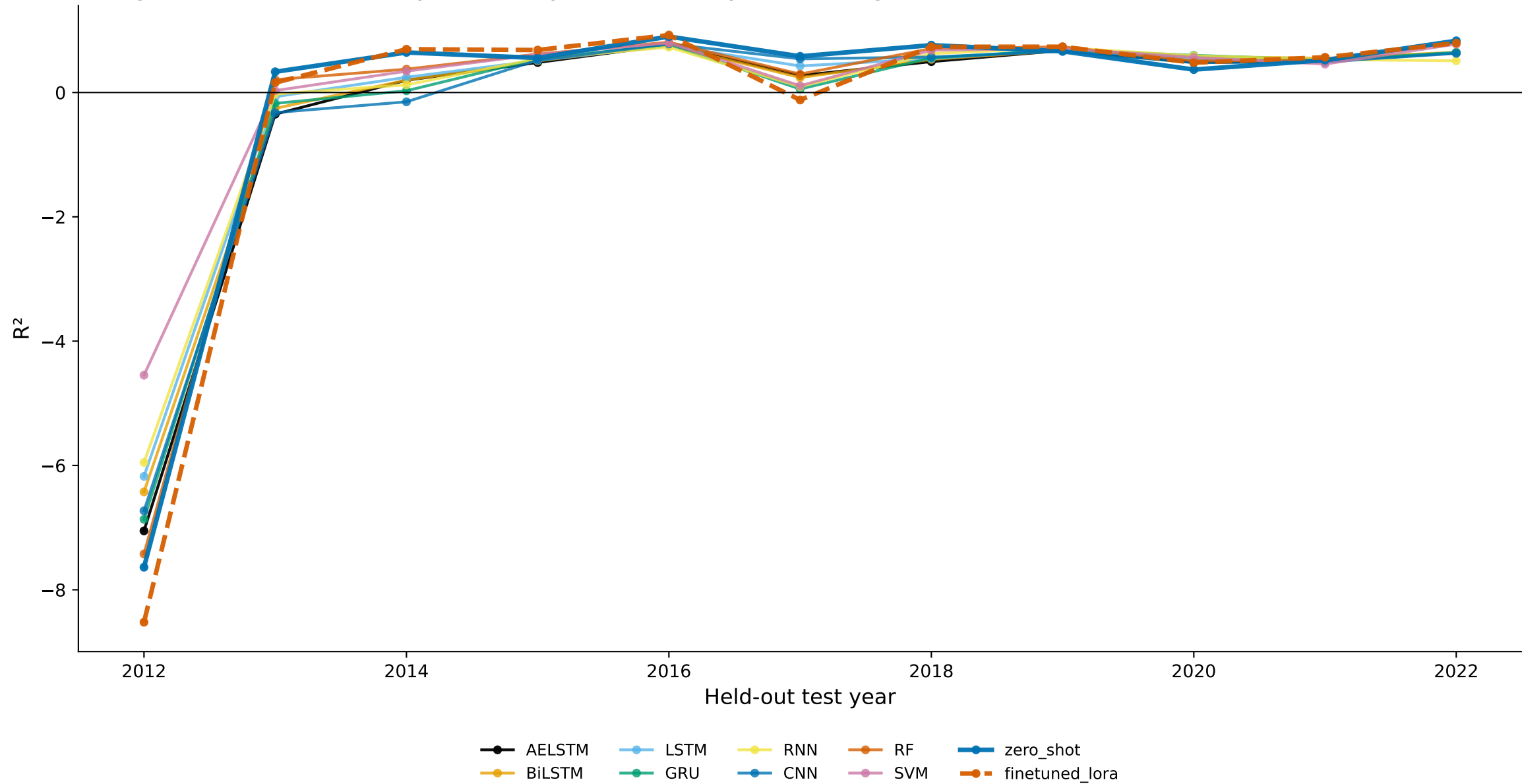
evergreen — LOYO-CV: R^2 by held-out year, fixed 12-year training window
