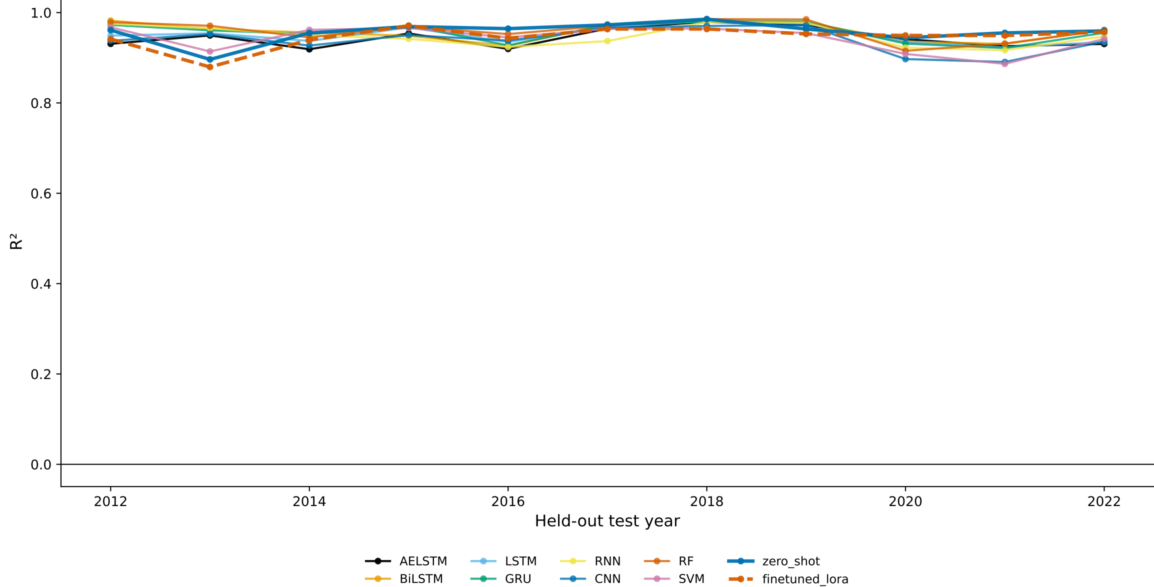
high_amplitude_deciduous — LOYO-CV: R^2 by held-out year, fixed 12-year training window
