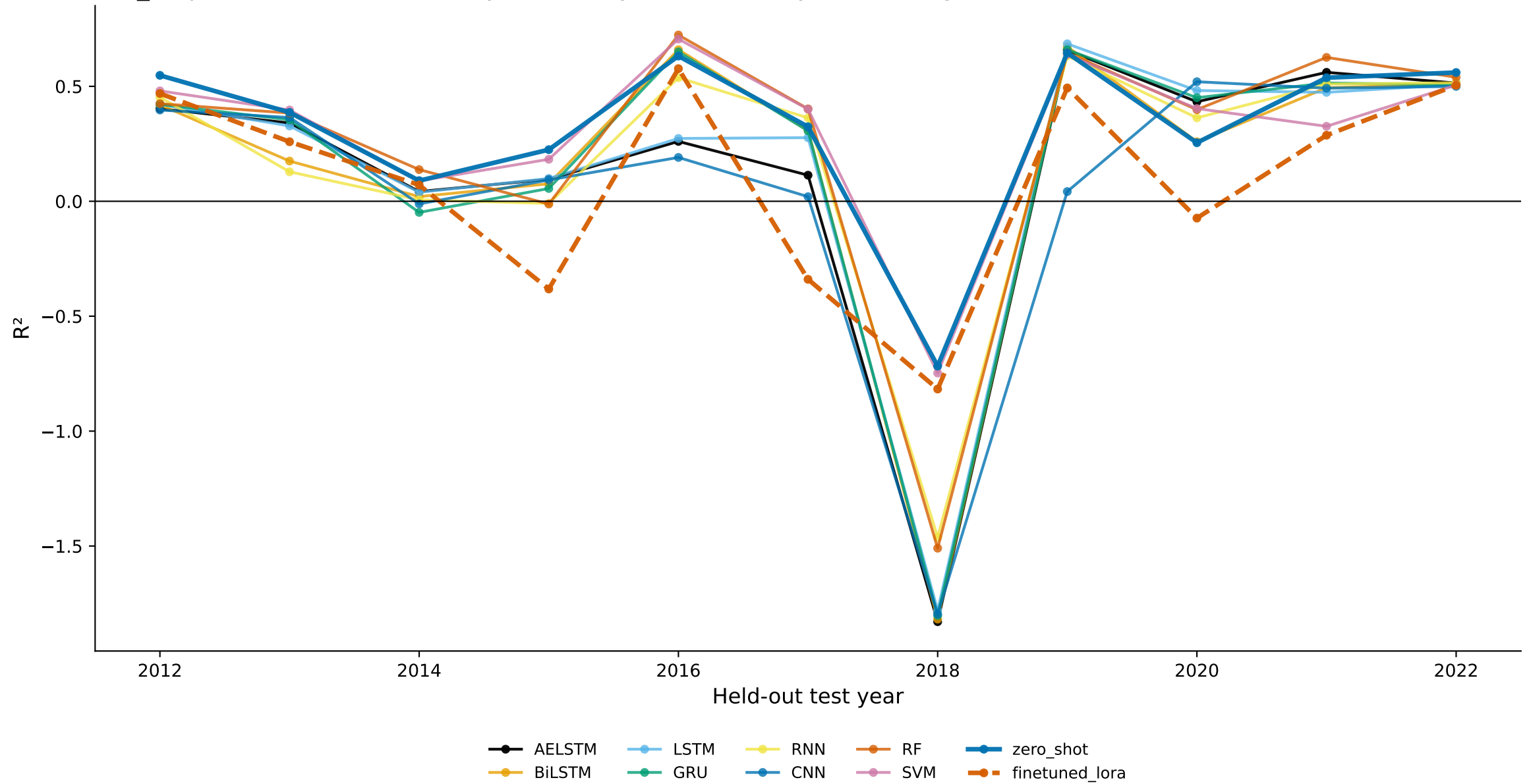
low_amplitude — LOYO-CV: R^2 by held-out year, fixed 12-year training window
