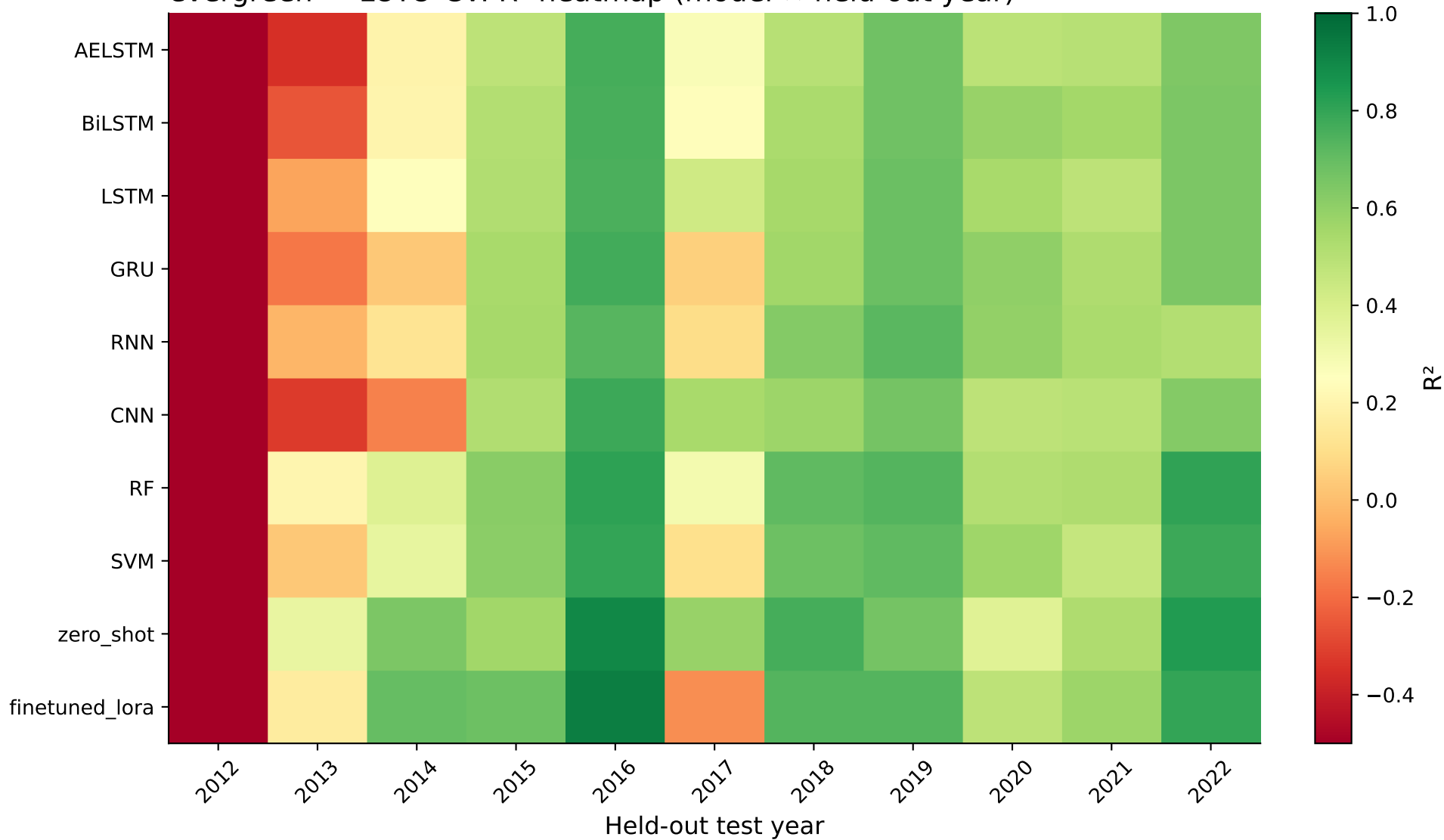
evergreen — LOYO-CV: R^2 heatmap (model \times held-out year)
