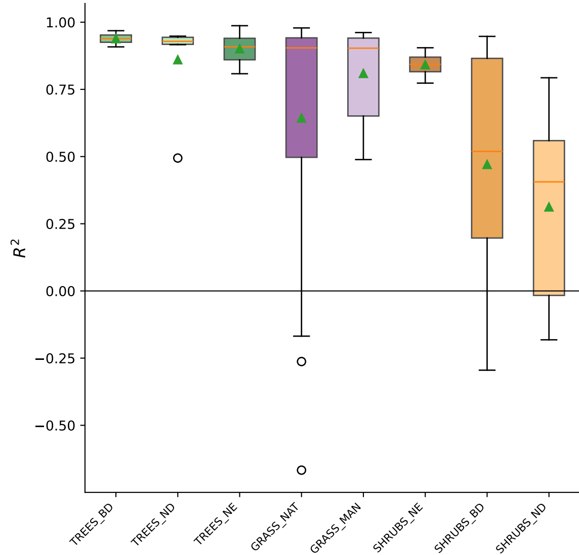
(b) By dominant vegetation class
