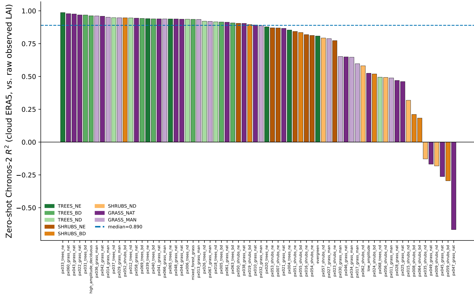
(a) All 70 pixels, sorted by R^2 (cloud ERA5, 22-yr context)
