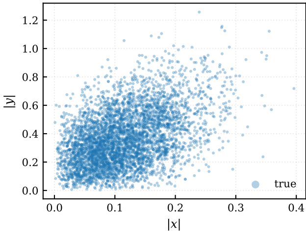
AM/AM — gmp_pa (test)
